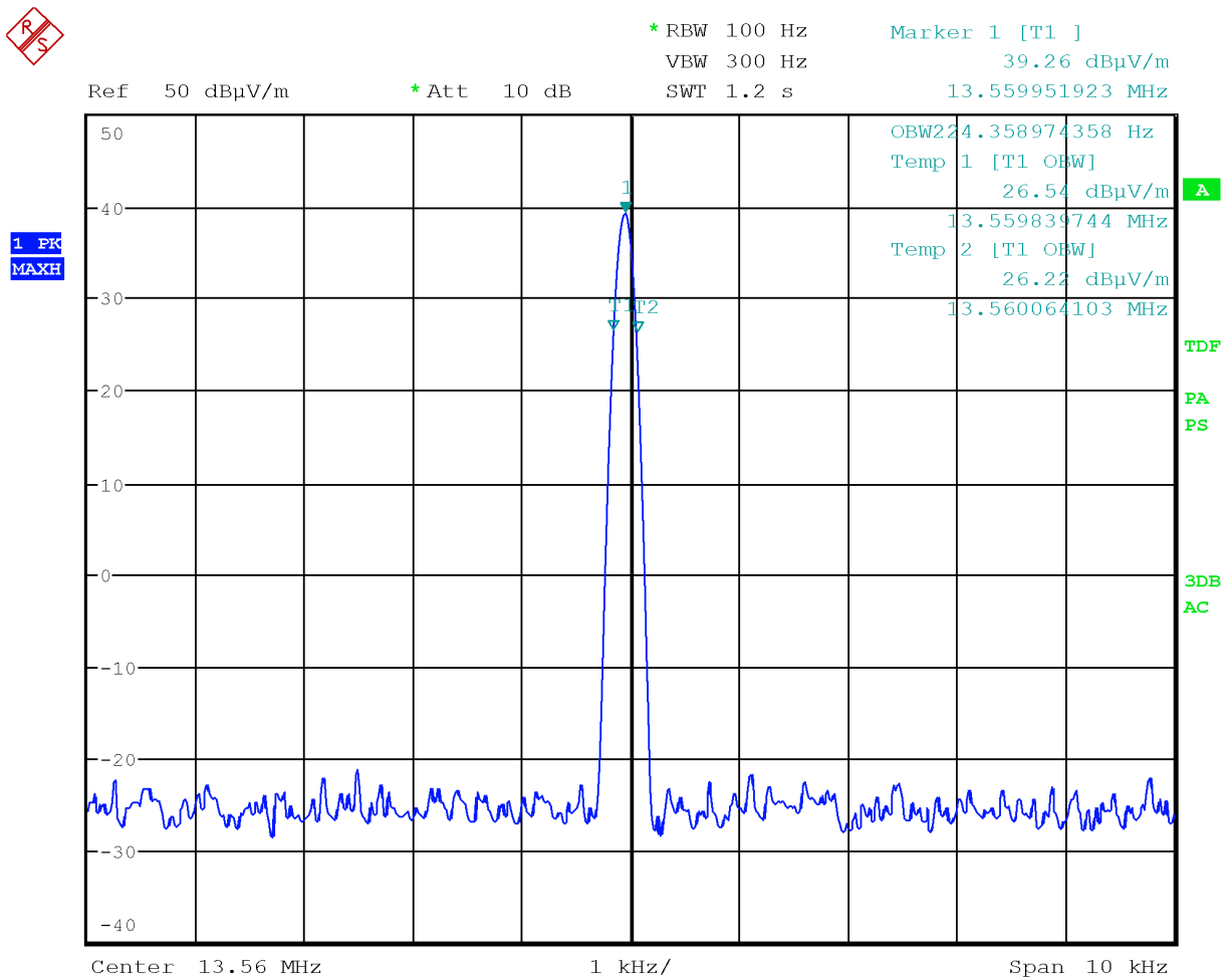
Figure 8.2-2: 99% dB bandwidth
