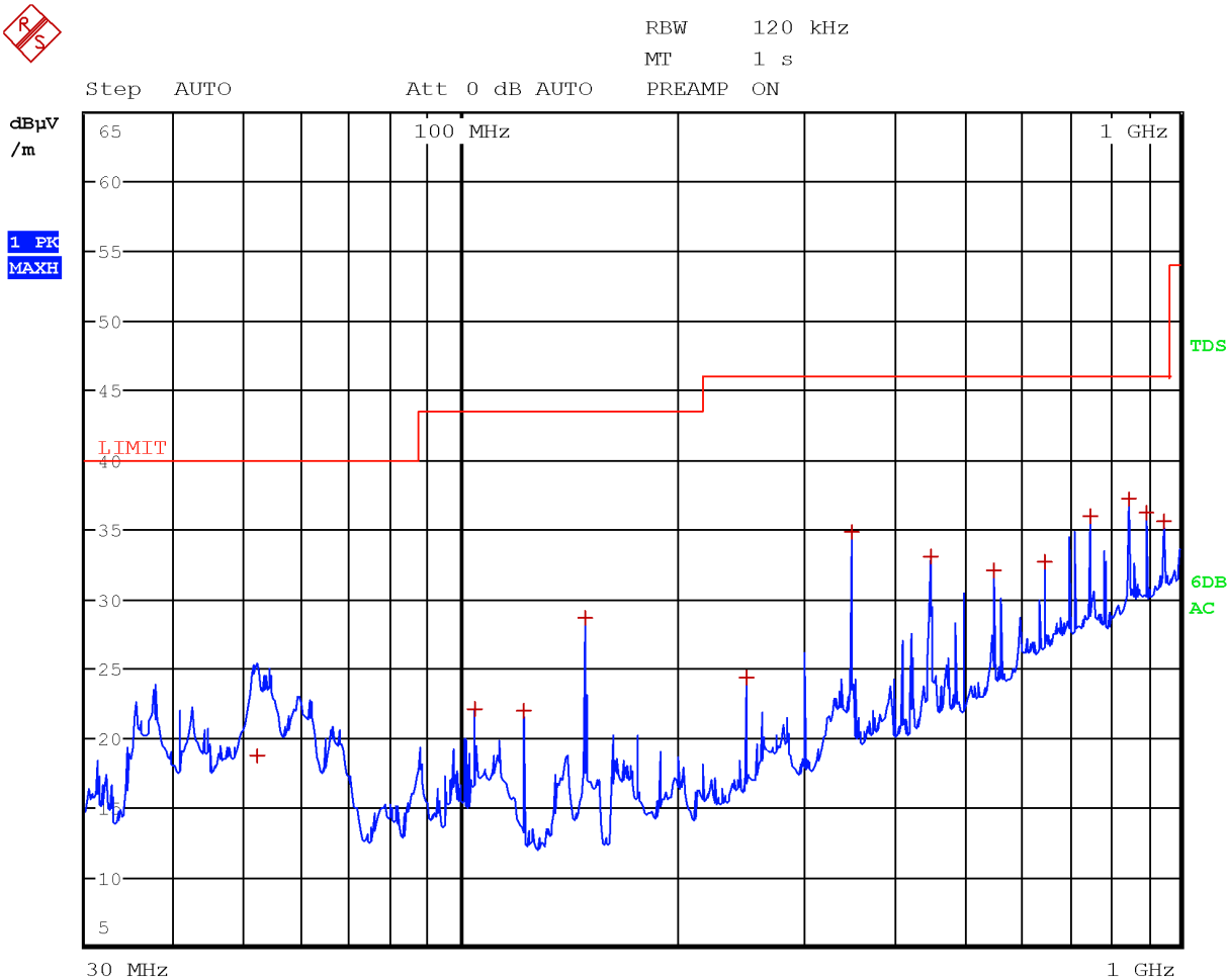
Figure 8.4-3: Field strength of spurious emissions above 30 MHz with antenna in vertical polarization
