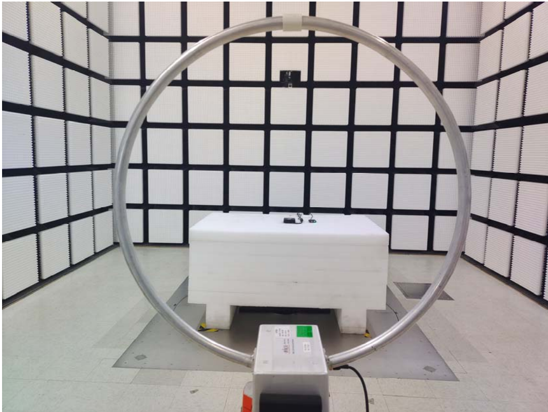
Radiated Emission Below 30MHz Perpendicular View
