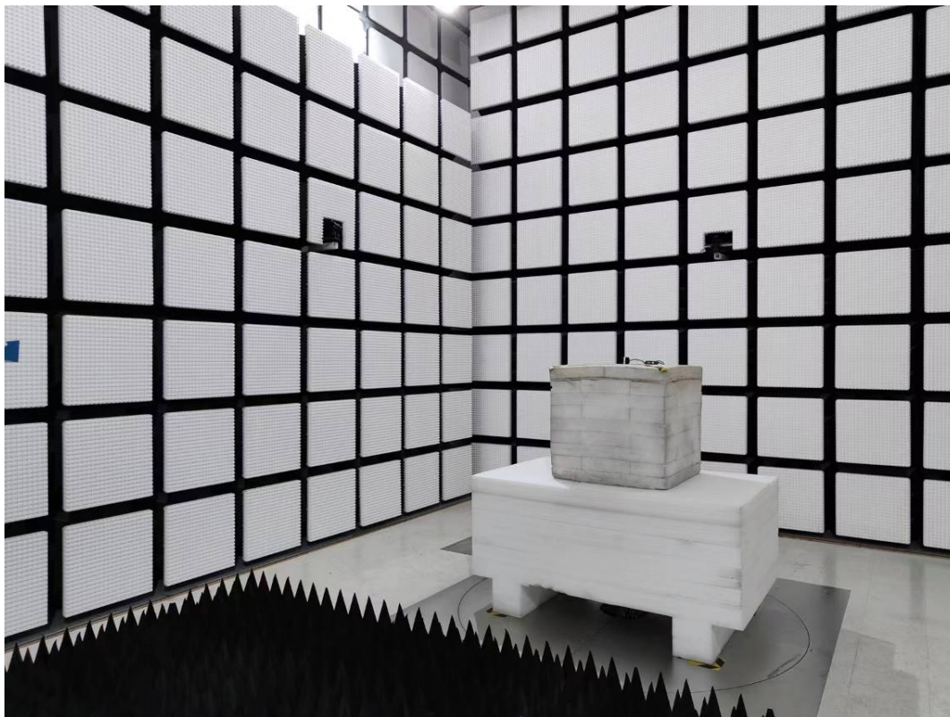
Radiated Emission Above 1GHz View 26.5G-40G
