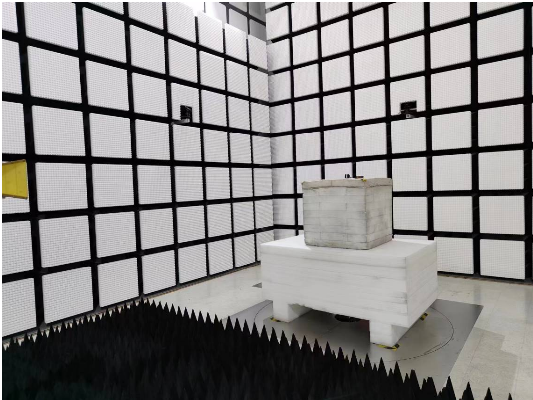
Radiated Emission Above 1GHz View 1G-18G
