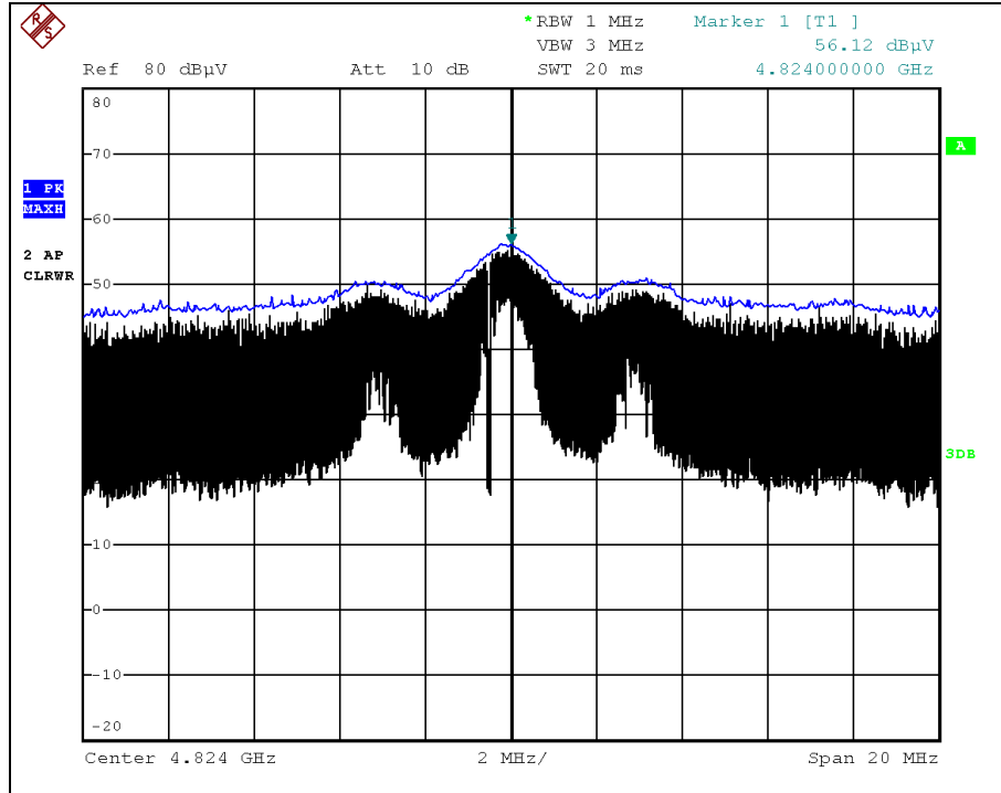
802.11b _ Low frequency Spurious - Average
