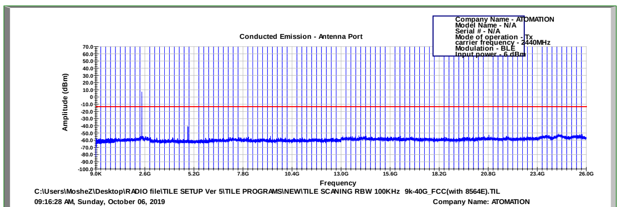
Figure 35 2440.0 MHz, BLE
