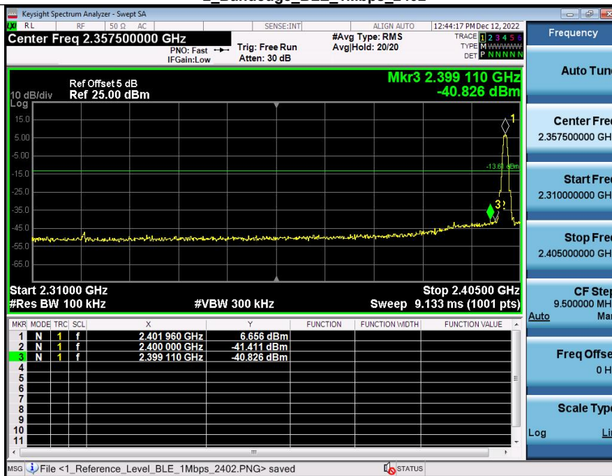
2 Bandedge_BLE_1Mbps_2402
