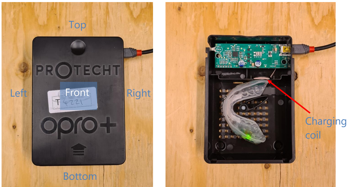
Figure 2 DUT lid closed and open
