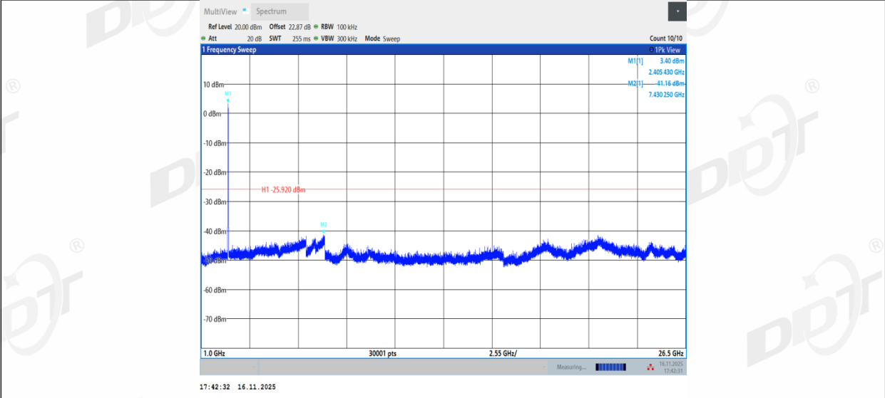
11N20SISO_Ant1_2437_0~Reference
