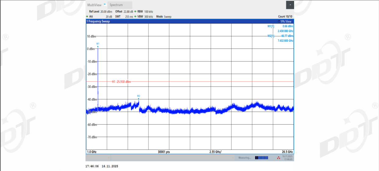
11N20SISO_Ant1_2462_0-Reference
