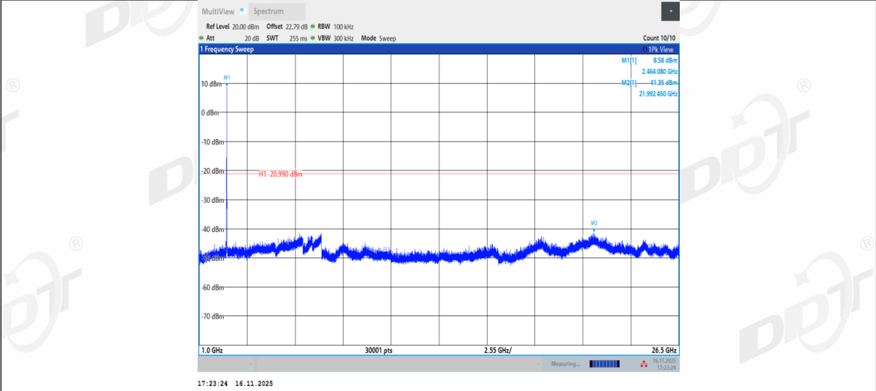
11G_Ant1_2412_0~Reference
