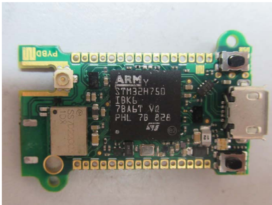
PYBD-SH0W – PCB Chip View
