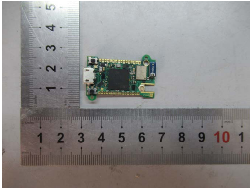
PYBD-SH3W – PCB Top View
