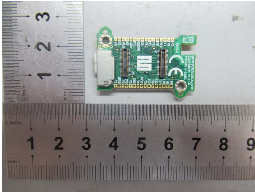
PYBD-SF3W – PCB Chip View
