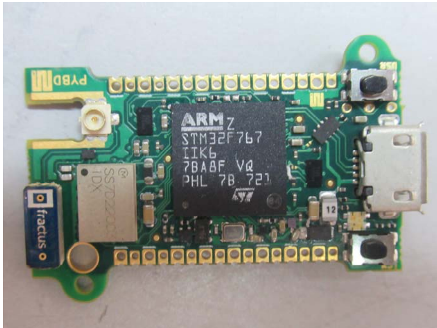
PYBD-SF6W – PCB Chip View
