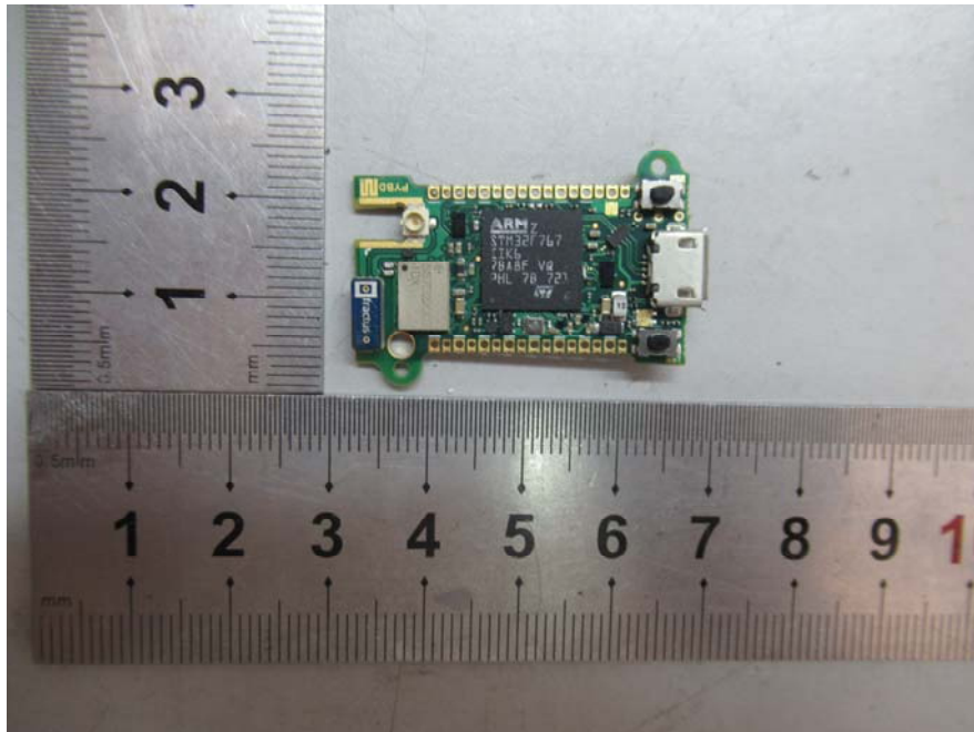
PYBD-SF6W – PCB Top View
