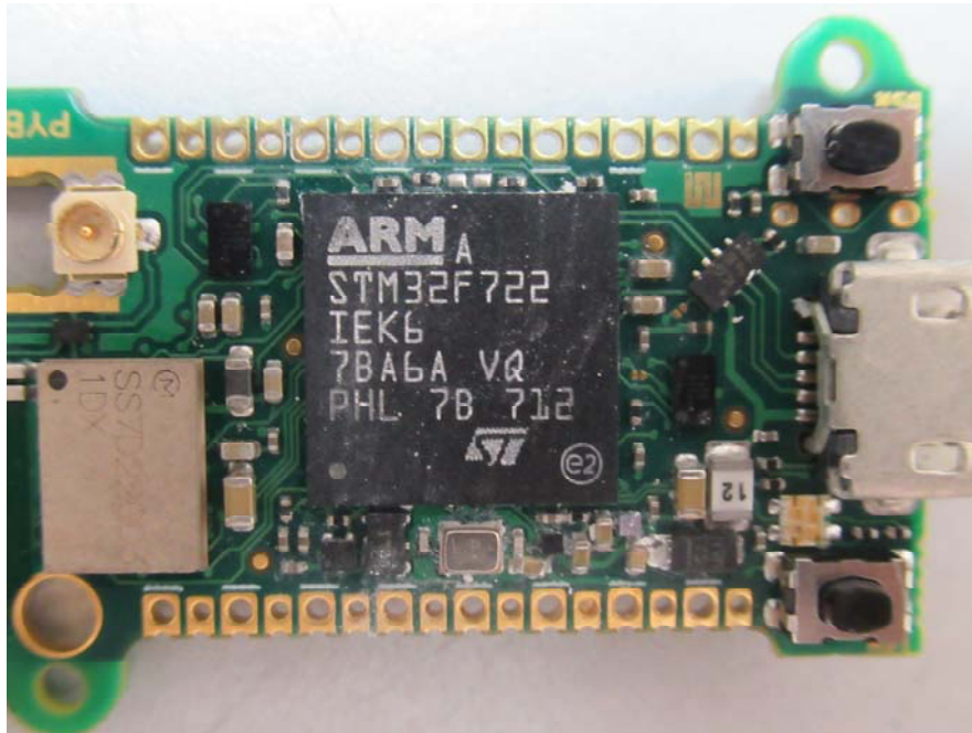
PYBD-SF2W – PCB Chip View
