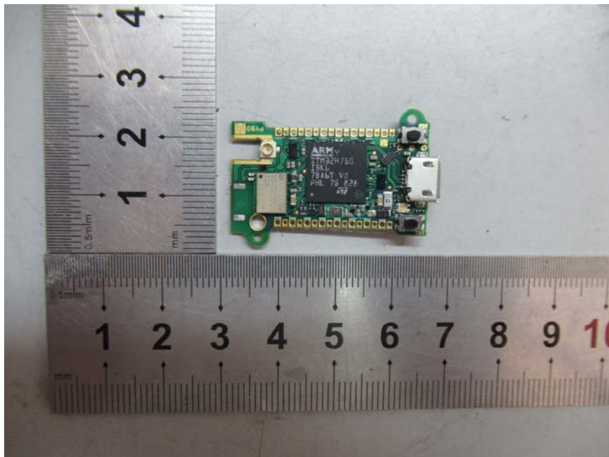
PYBD-SH0W – PCB Top View
