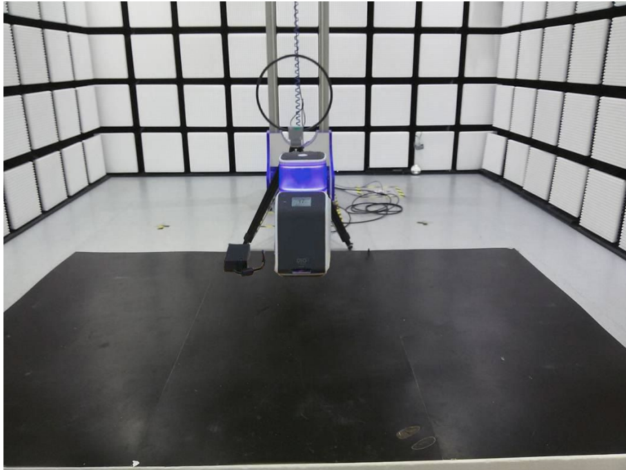
Radiated Measurement Photos (Below 30MHz)
