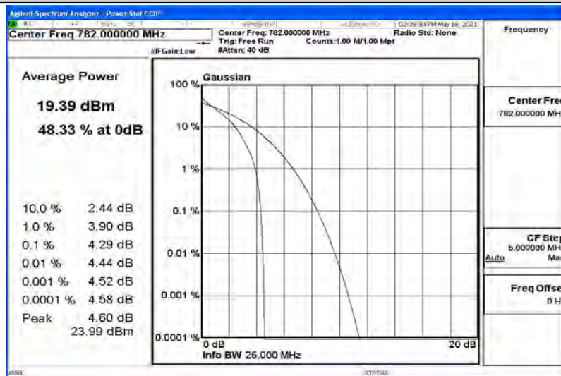
Band13-5MHz-QPSK-23255-25RB#0
