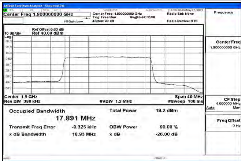
Band2-20MHz-16QAM-19100-100RB#0-17.891
