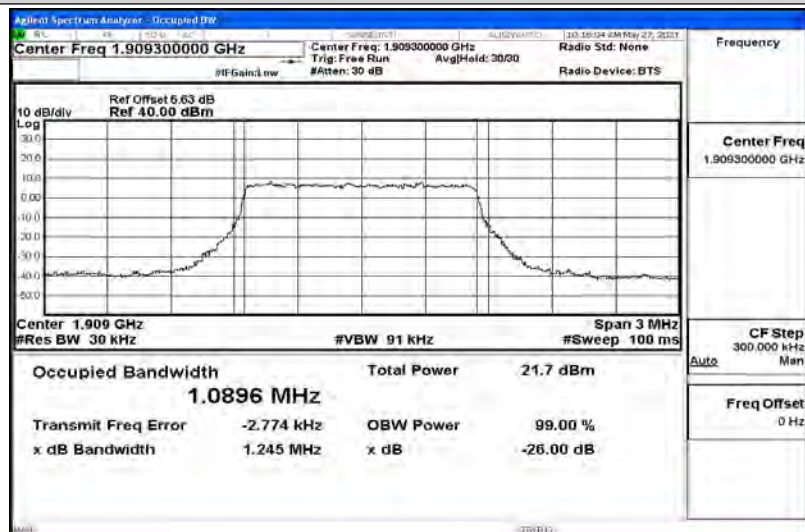
Band2-1.4MHz-QPSK-19193-6RB#0-1.0896
