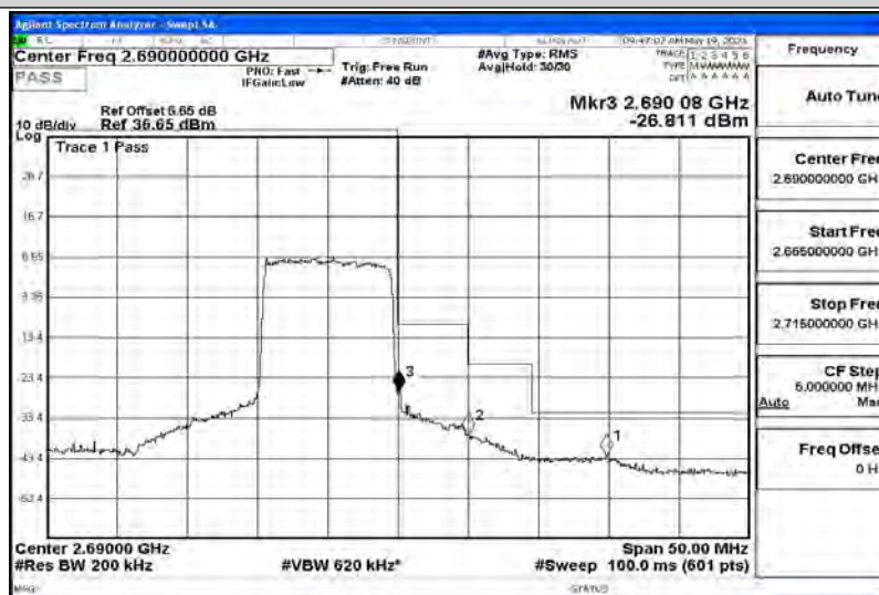
Band41-10MHz-16QAM-39700-50RB#0
