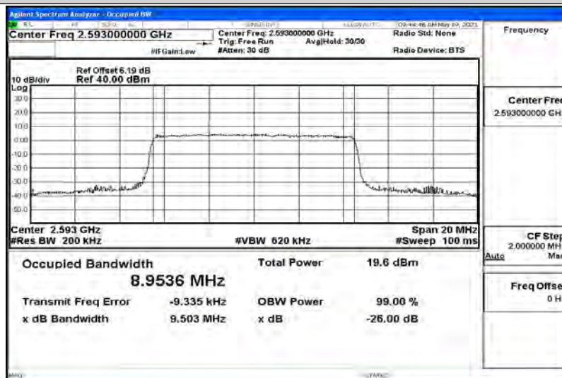
Band41-10MHz-16QAM-41540-50RB#0-8.9580
