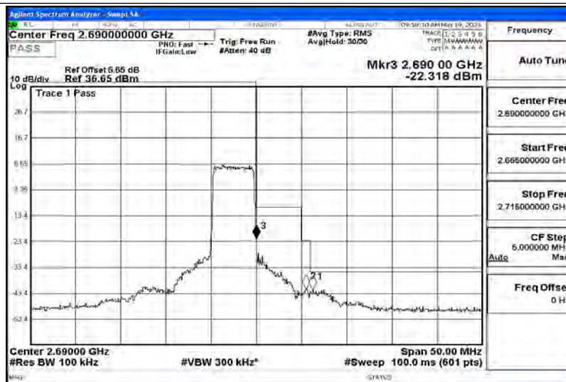
Band41-5MHz-16QAM-39675-25RB#0
