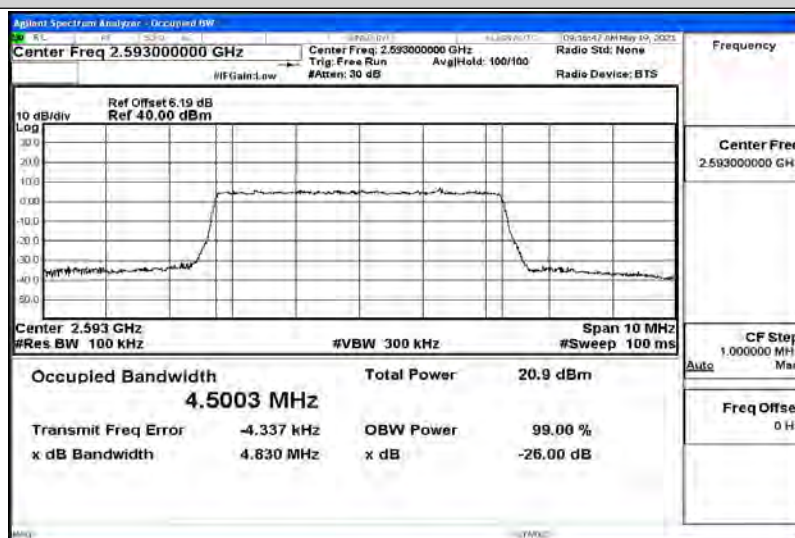
Band41-5MHz-16QAM-41565-25RB#0-4.4936
