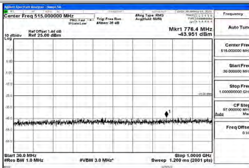
Band41-20MHz-16QAM-39750-1RB#0-Range2:1000~10000MHz
