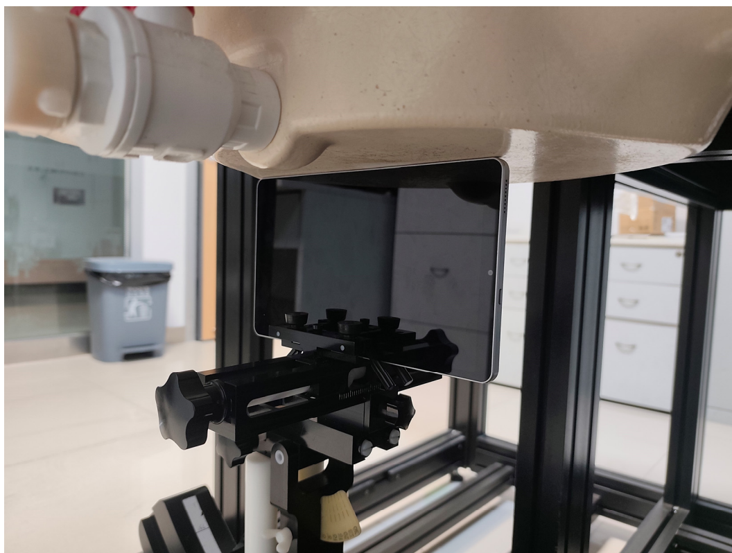
WWAN ANT Body Top Setup Photo (0 mm)
