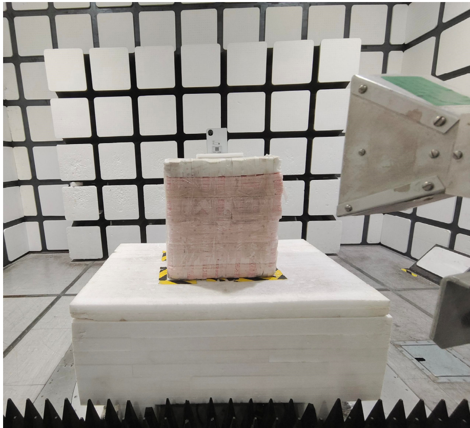
Radiated Emissions View (18-40 GHz)
