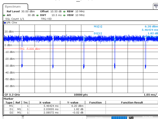
802.11a_5200MHz
