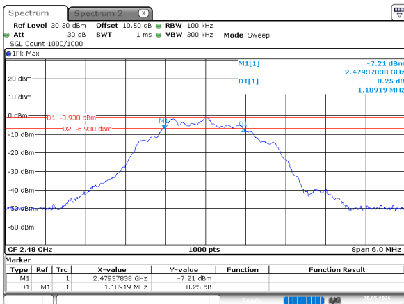
BLE_2M_High_Channel
