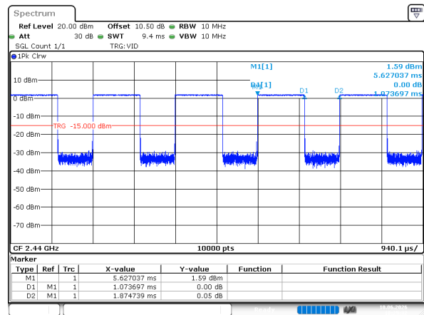
BLE_2M_Middle_Channel
