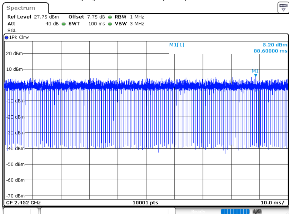
Duty Cycle NVNT 802.11n(HT40) 2452MHz
