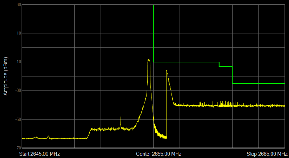
Band41 QPSK BW=5MHz Channel=41215 RB Size=1 Position=#Max
