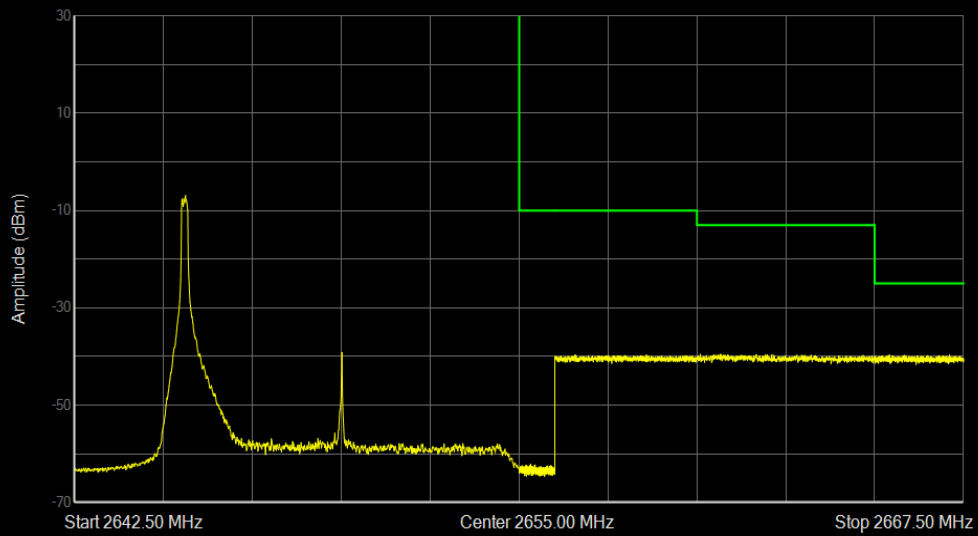
Band41 QPSK BW=10MHz Channel=41190 RB Size=1 Position=#0
