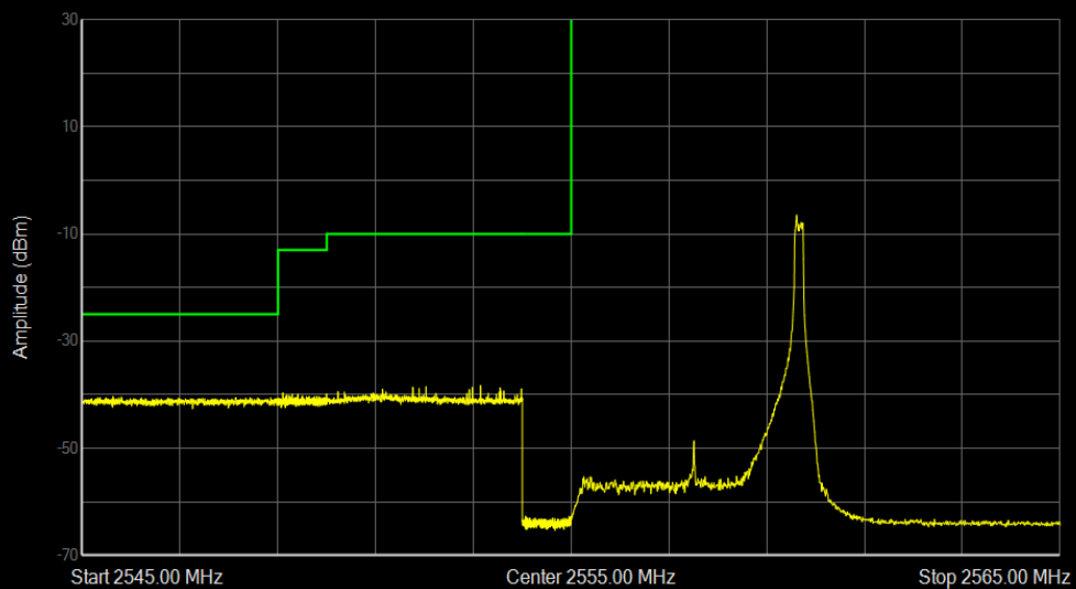
Band41 QPSK BW=5MHz Channel=40265 RB Size=1 Position=#Max
