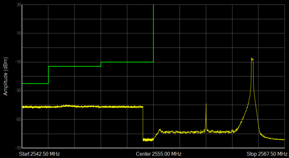
Band41 QPSK BW=10MHz Channel=40290 RB Size=1 Position=#Max
