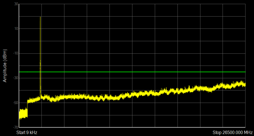
Band7 QPSK BW=15MHz Channel=20825 RB Size=75 Position=#0
