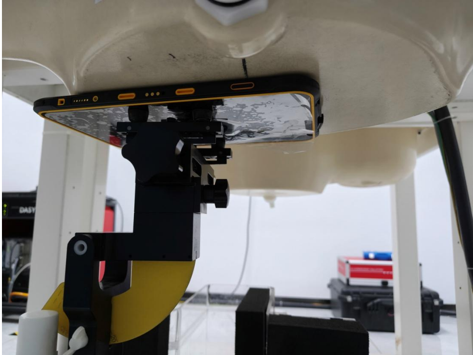
Body Back(WWLN/BT) Setup Photo (0mm)
