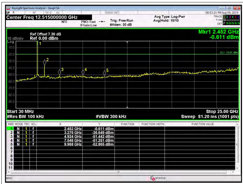
(802.11 HT20, Channel = 11, 30MHz to 25GHz;ANT0)
