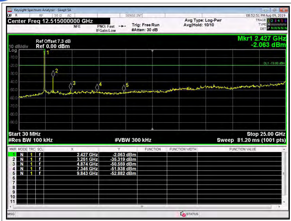
(802.11 HT20, Channel = 6, 30MHz to 25GHz;ANT0)
