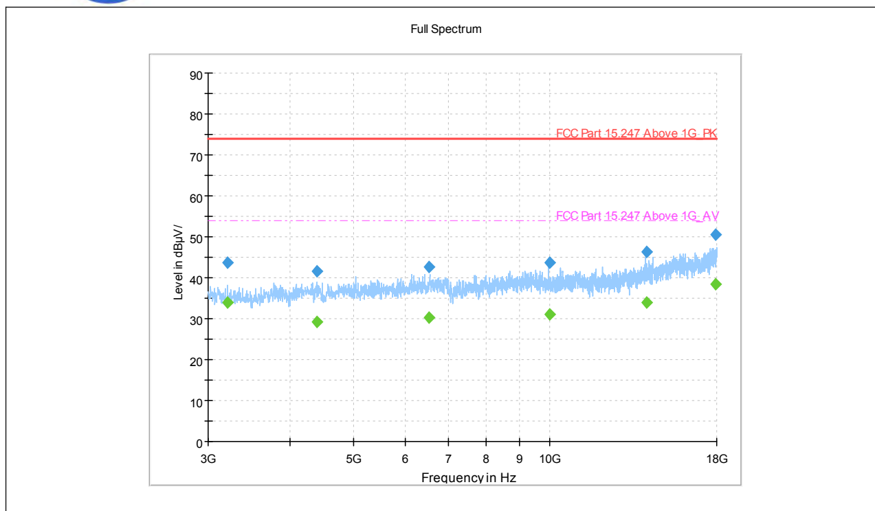
(802.11g _2412MHz, Antenna Horizontal, 3GHz to 18GHz)
