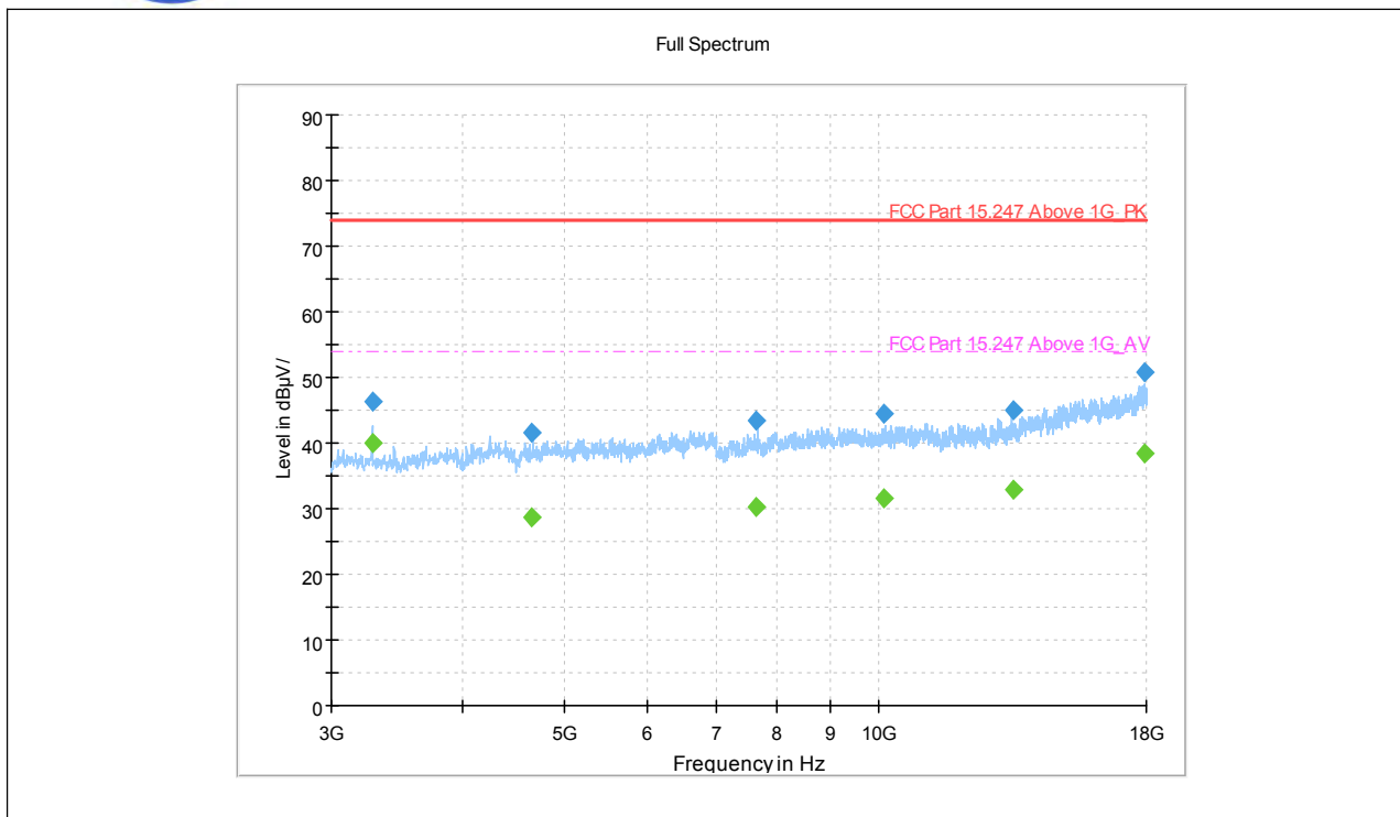
(802.11n_20M_2462MHz, Antenna Vertical, 3GHz to 18GHz)
