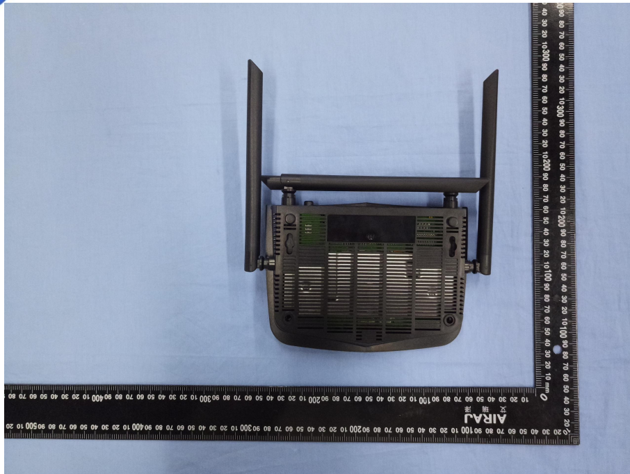
EUT unit bottom view
