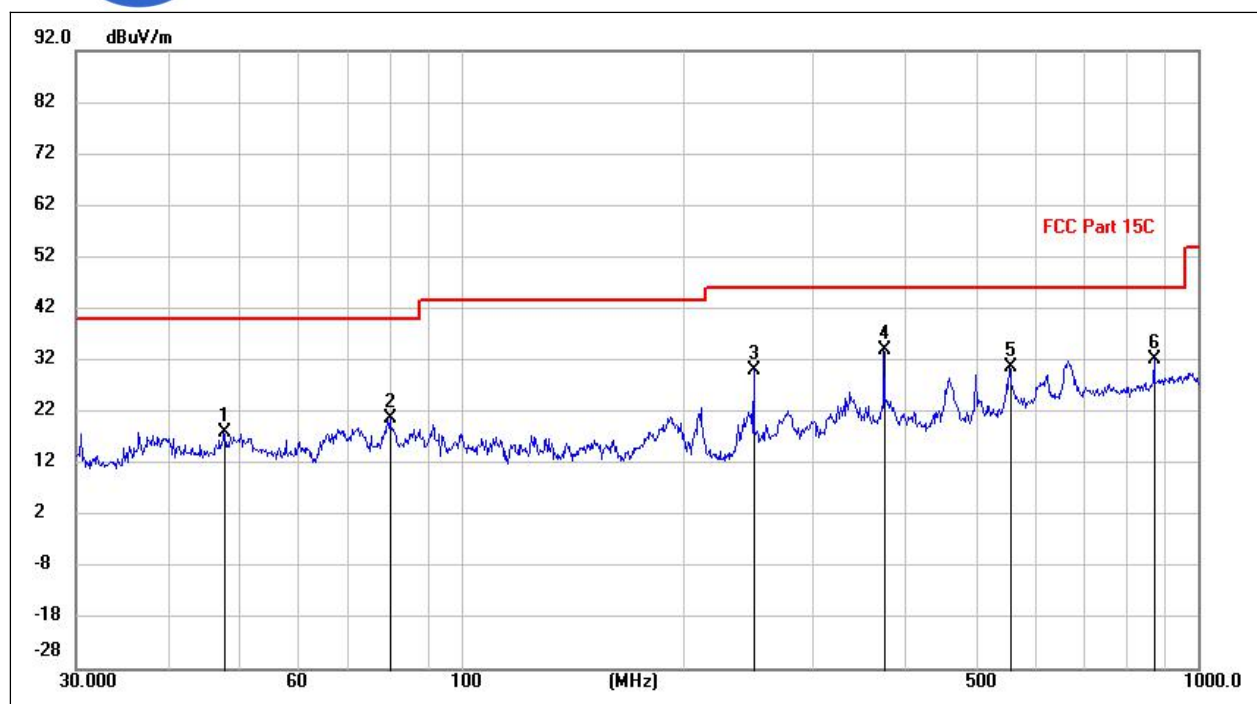
(802.11ac_5785MHz, Antenna Vertical, 30MHz to 1GHz)
