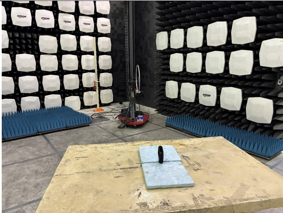
Radiated Emissions 9 kHz – 30 MHz Rear View
