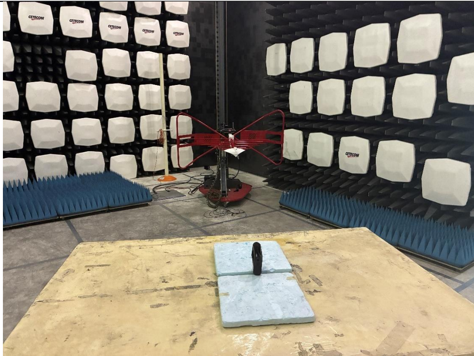
Radiated Emissions 30 MHz – 1 GHz Rear View
