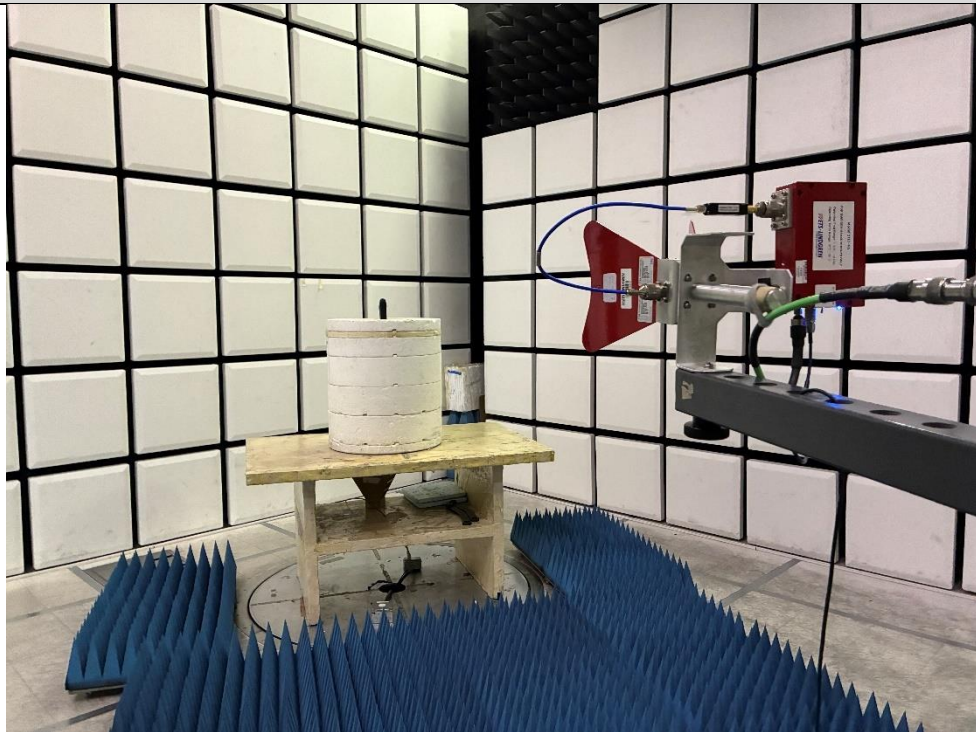
Radiated Emissions 3 GHz – 18 GHz Rear View
