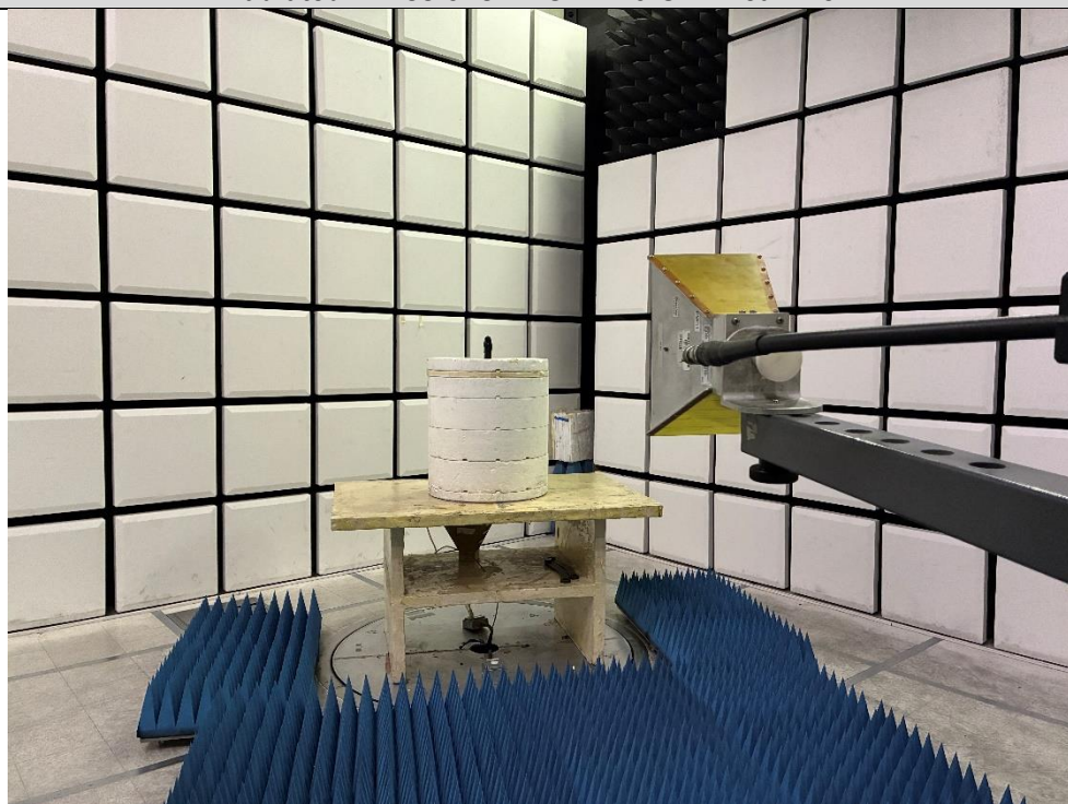
Radiated Emissions 1 GHz – 3 GHz Rear View
