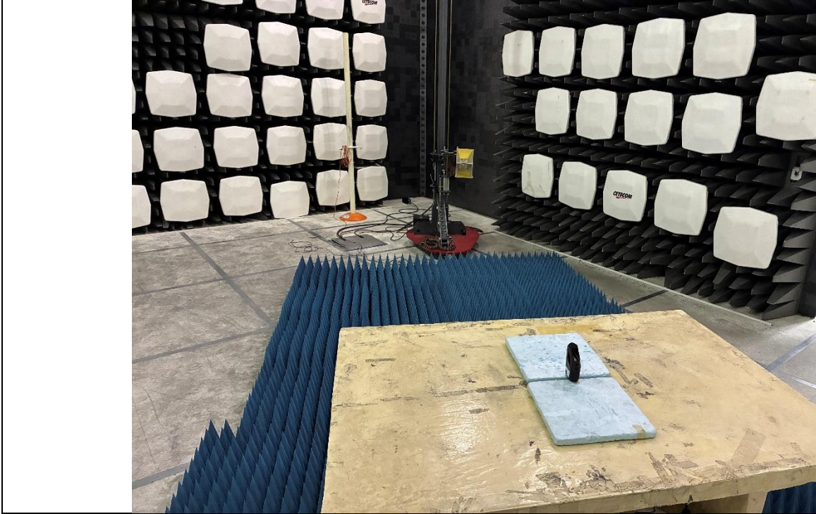
Radiated Emissions 1 GHz – 3 GHz Rear View
