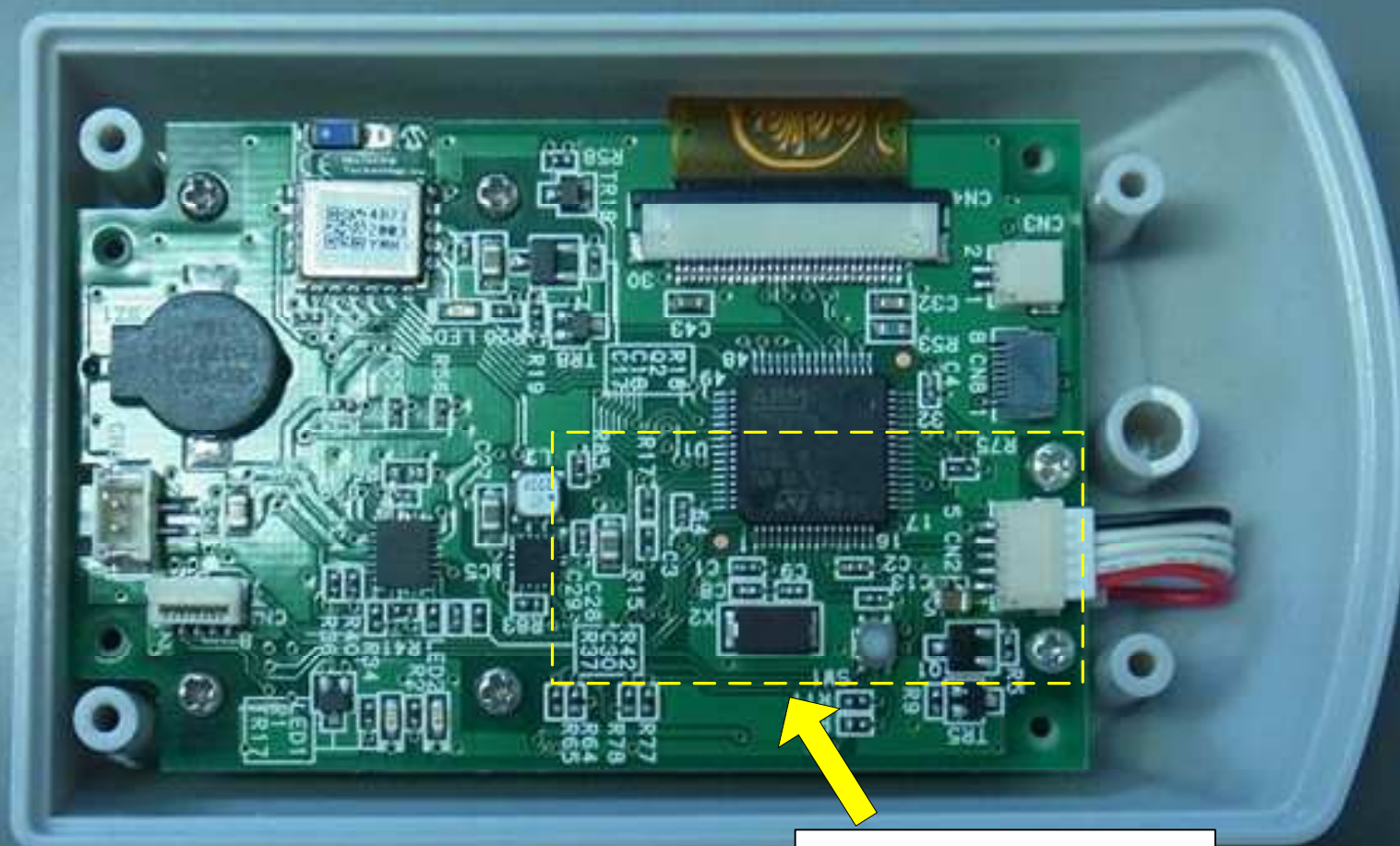
RFID Module (Back side of board)
