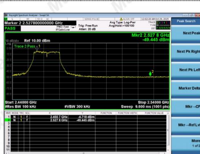
Right bandedge
