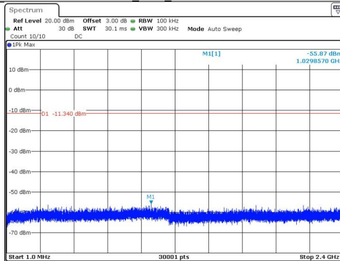
11B_2462_1~2400
