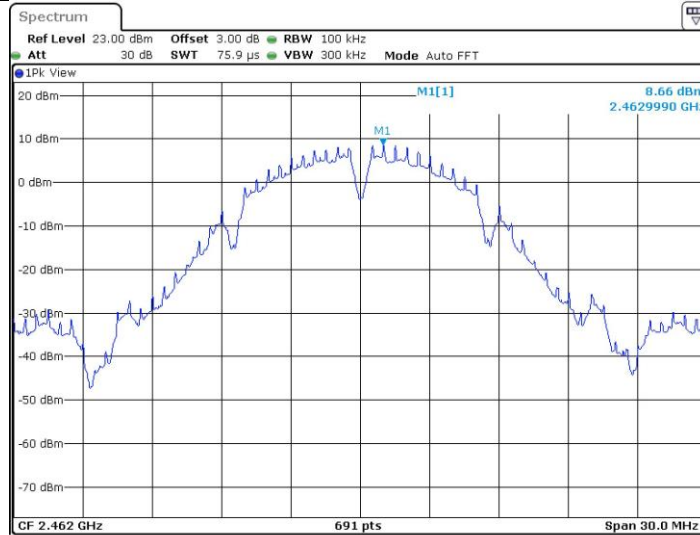
11B_2462_0~Reference
