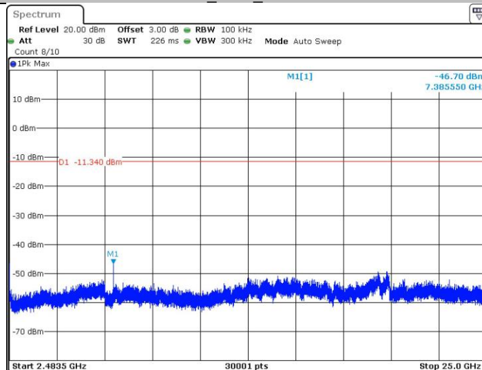
11B_2462_2483.5~25000
