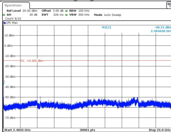
11G_2462_2483.5-25000
