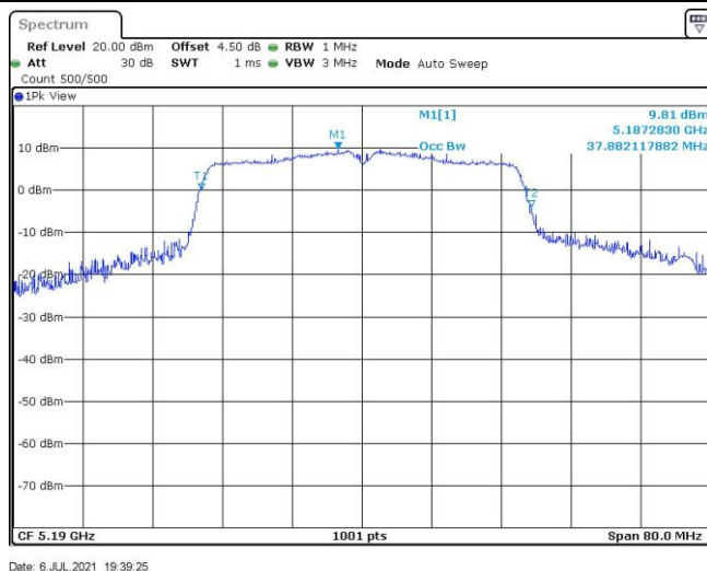
11N40SISO_Ant1_5190
