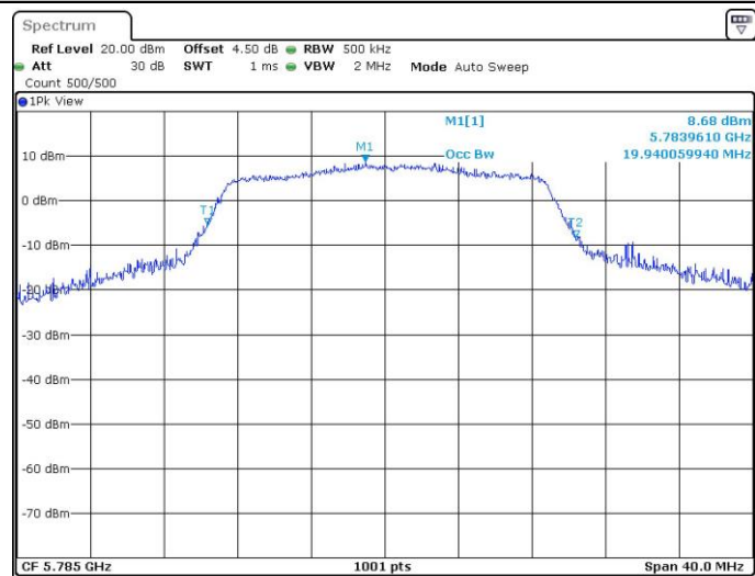
11AC20SISO_Ant1_5785
