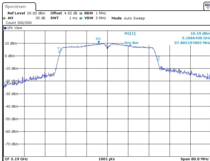
11AC40SISO_Ant1_5190
