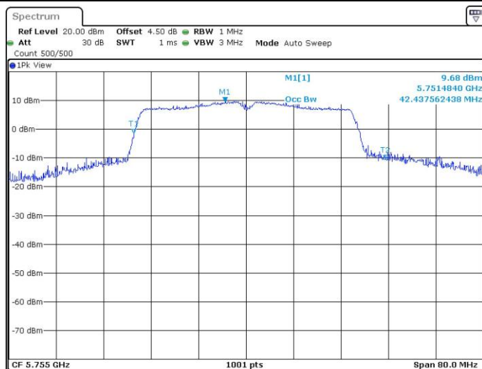
11AC40SISO_Ant1_5755
