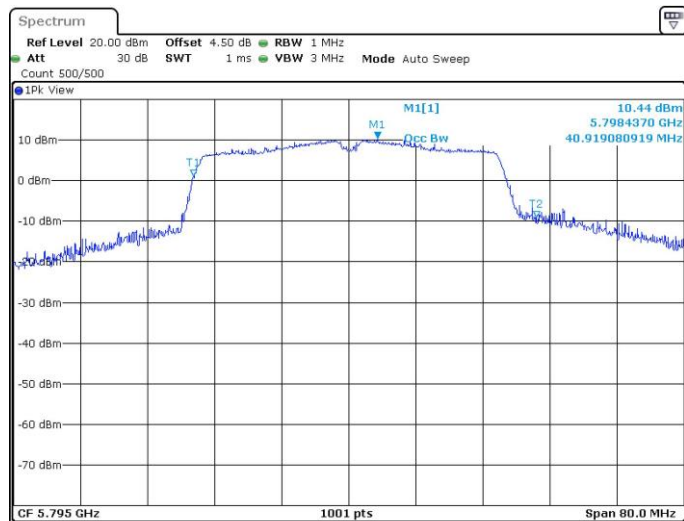
11AC40SISO_Ant1_5795
