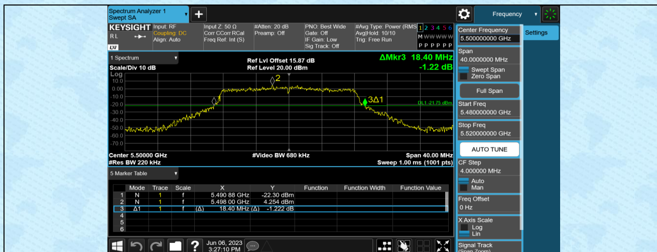
11A-CDD-Ant1-5500
