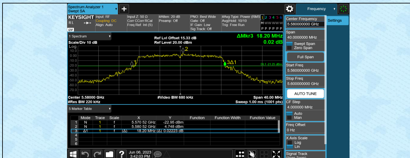
11A-CDD-Ant2-5580
