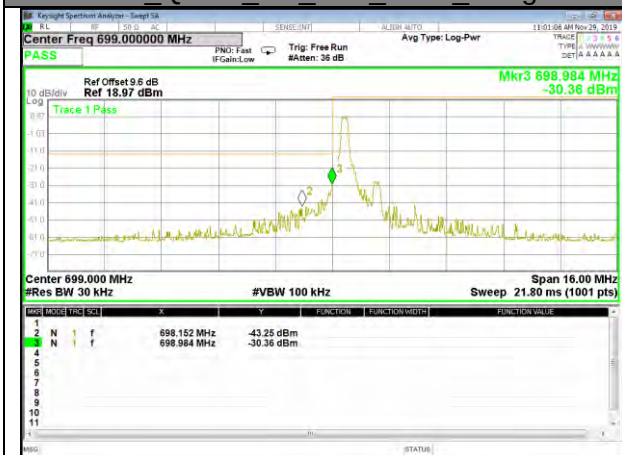
B12_QPSK_5M_Low_1-RB_Bedge
