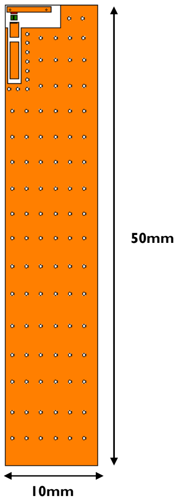
Fig. 7 Outlook and dimension of evaluation board (Scenario 2)
