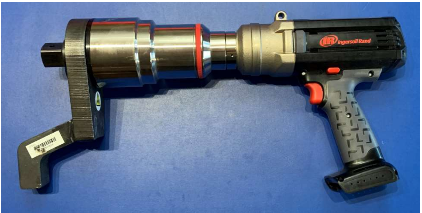
Pistol Tool QX5PM (with 4000Nm gearing)
