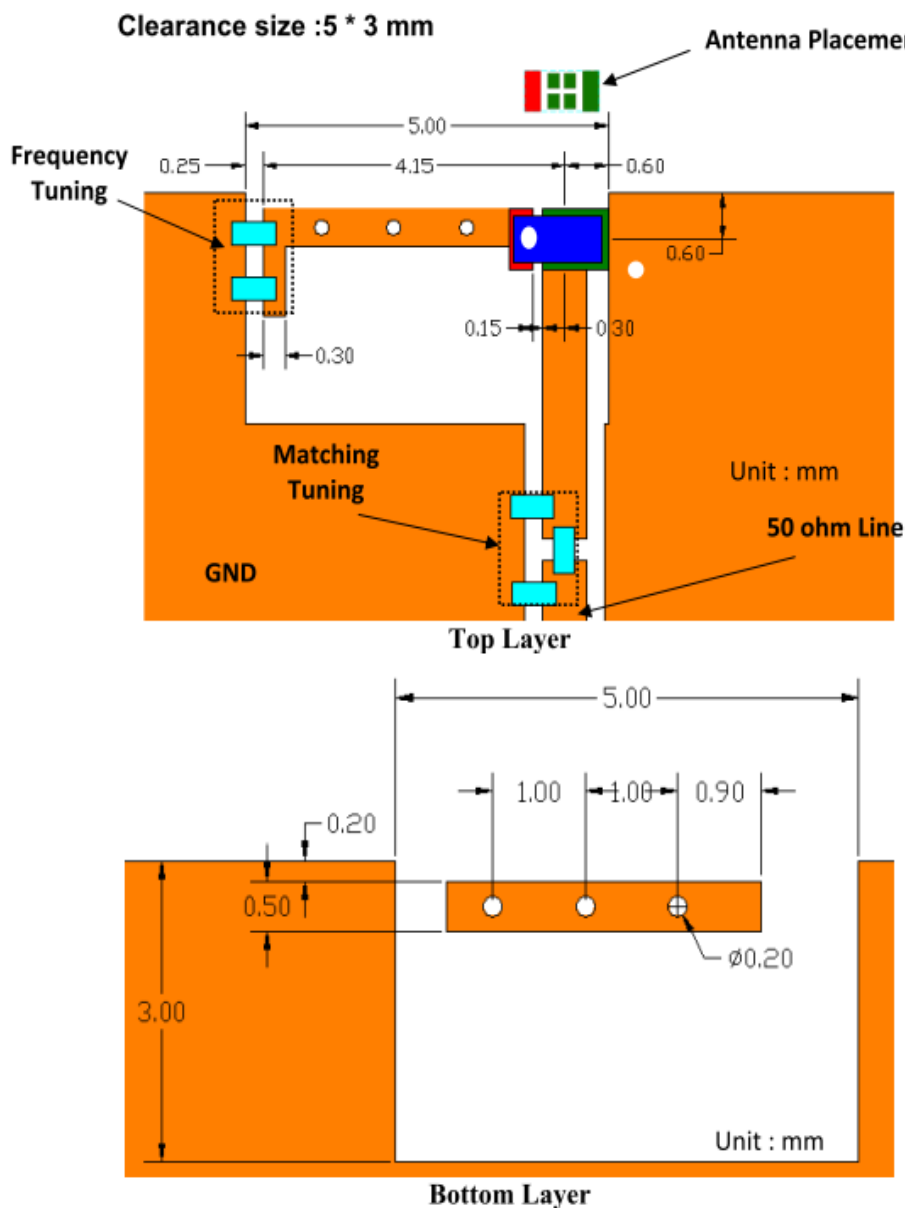
Details of soldering Pad of Scenario 1
