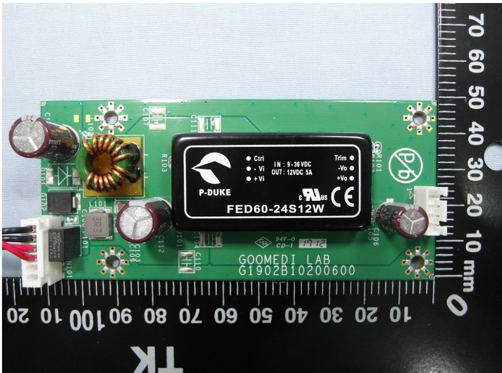
(35) EUT Photo
