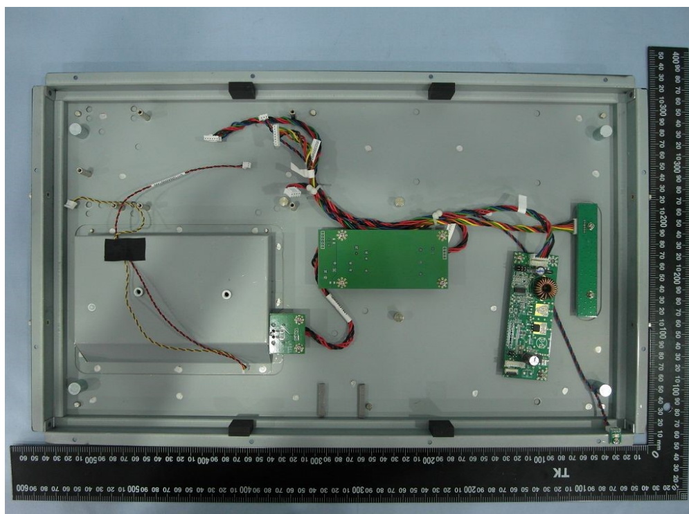
(29) EUT Photo
