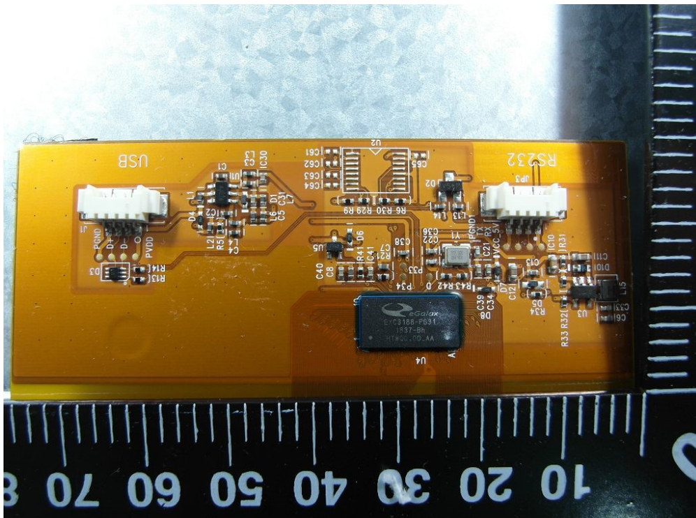
(51) EUT Photo
