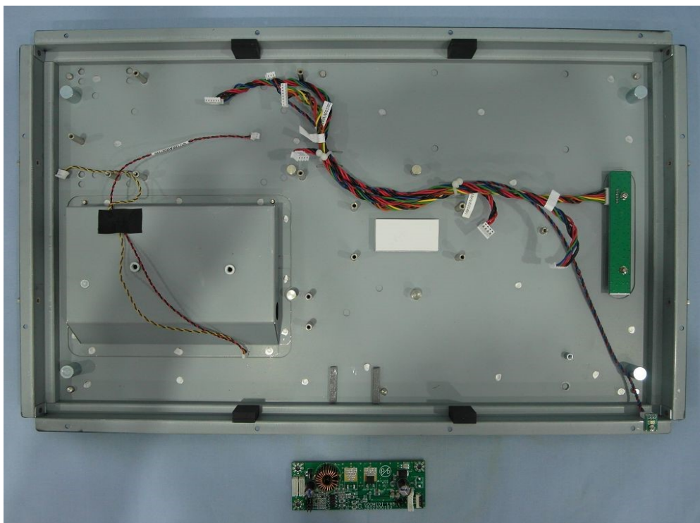
(39) EUT Photo
