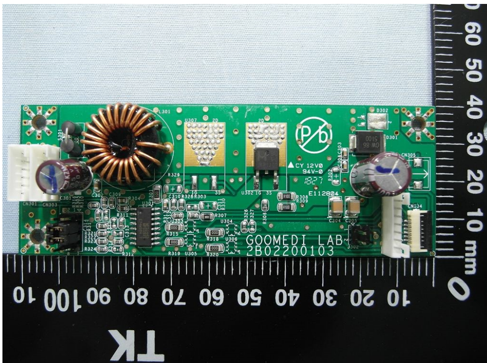
(39) EUT Photo
