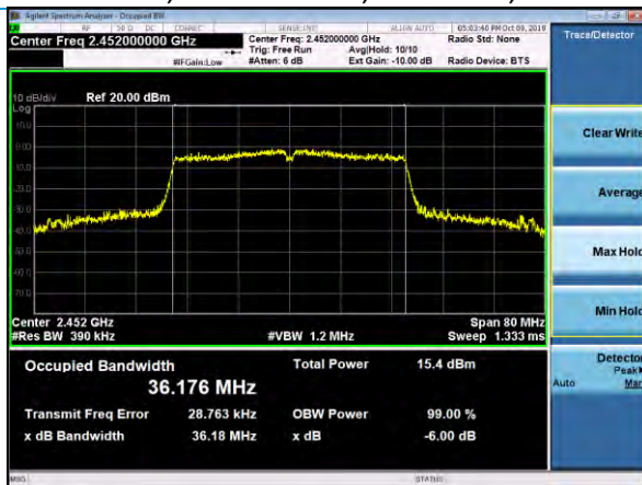
99% BW, 802.11n HT40, Channel9, MCS0
