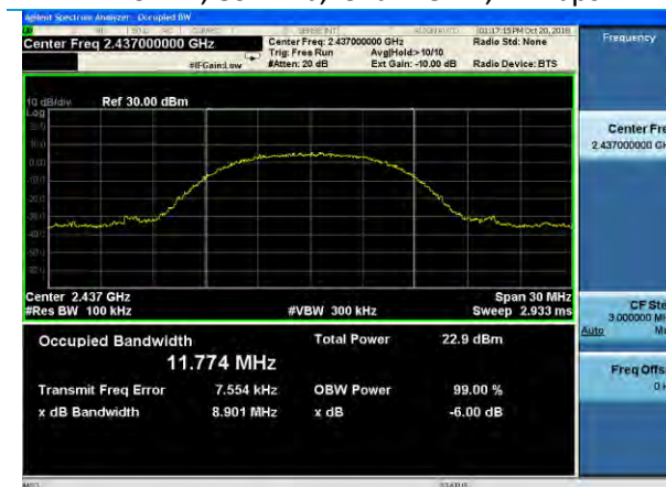
DTS BW, 802.11b, Channel 6, 11 Mbps
