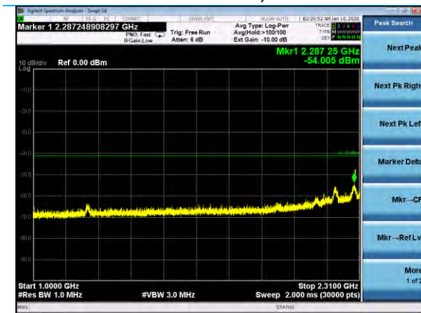
HT20 MCS0 Channel 6, 1-2.31 GHz
