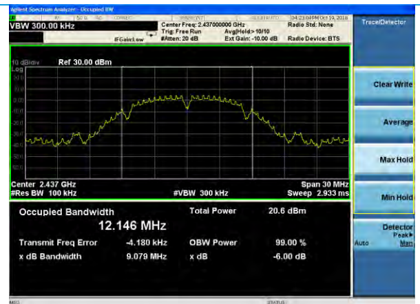
DTS BW, 802.11b, Channel 6, 1 Mbps
