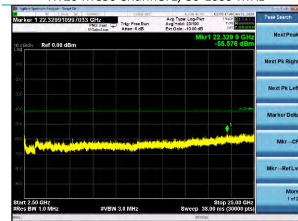
HT20 MCS0 Channel 1, 2.5-25 GHz
