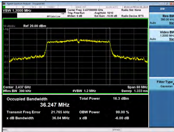
99% BW, 802.11n HT40, Channel6, MCS7
