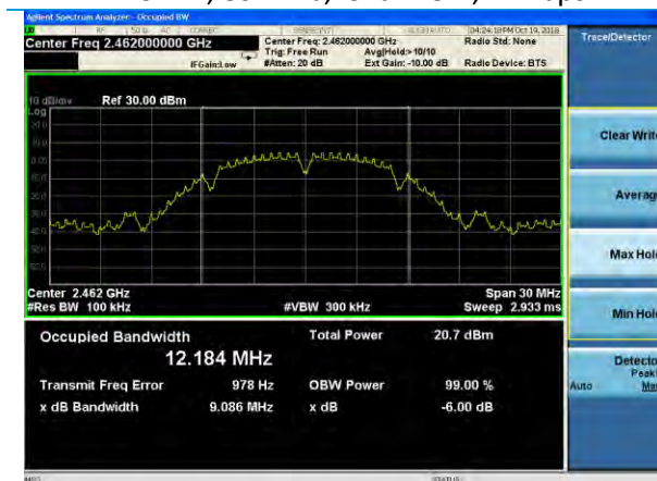
DTS BW, 802.11b, Channel 11, 1 Mbps
