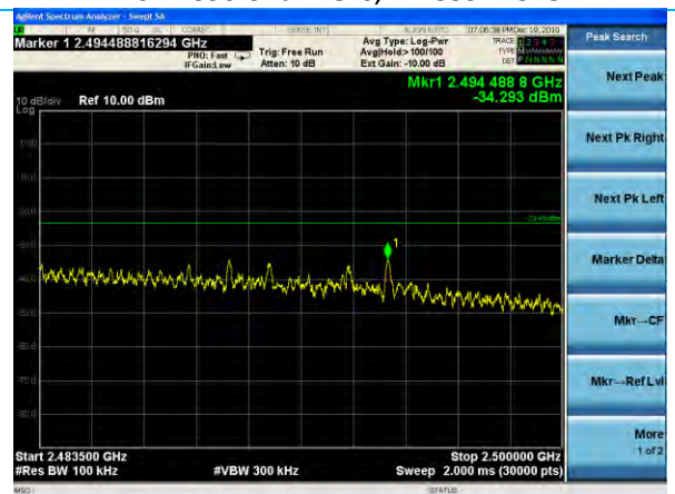
HT40 MCS0 Channel 9, 2.4835-2.5 GHz
