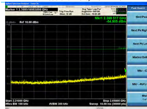
HT40 MCS0 Channel 9, 2.31-2.4 GHz
