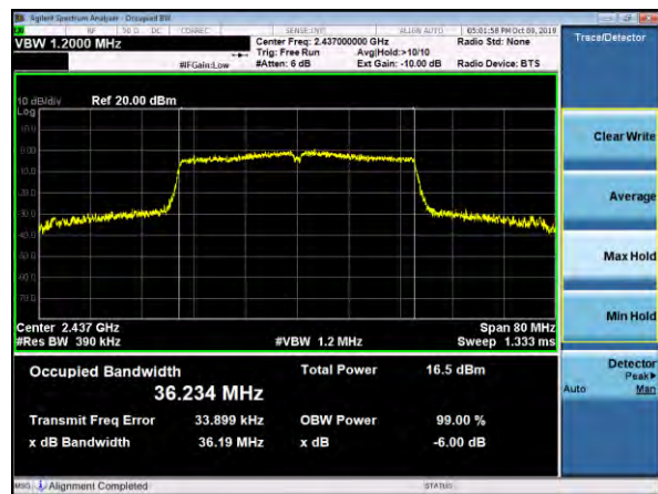
99% BW, 802.11n HT40, Channel6, MCS0
