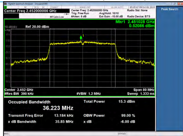
99% BW, 802.11n HT40, Channel9, MCS7
