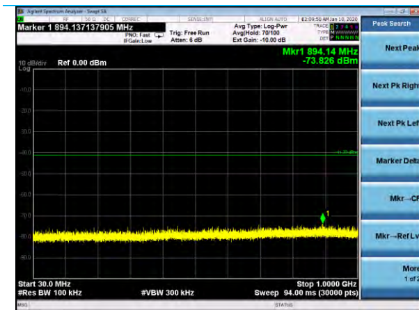
HT20 MCS0 Channel 1, 30-1000 MHz
