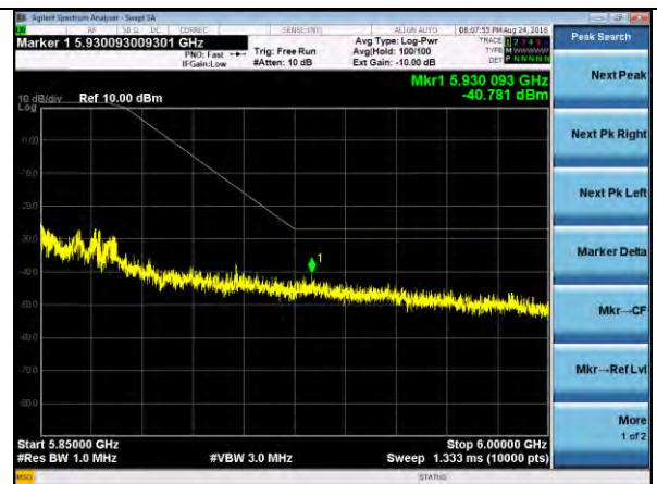
MCS9 UBE
