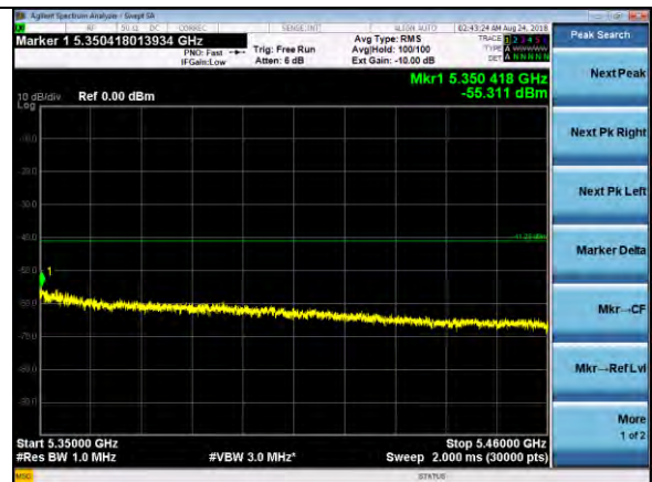
MCS9 UBE
