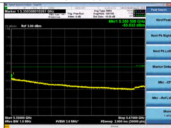
MCS0 UBE
