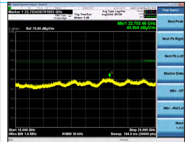
18 – 25 GHz
