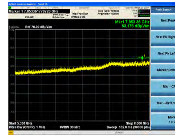
5.35 – 8 GHz
