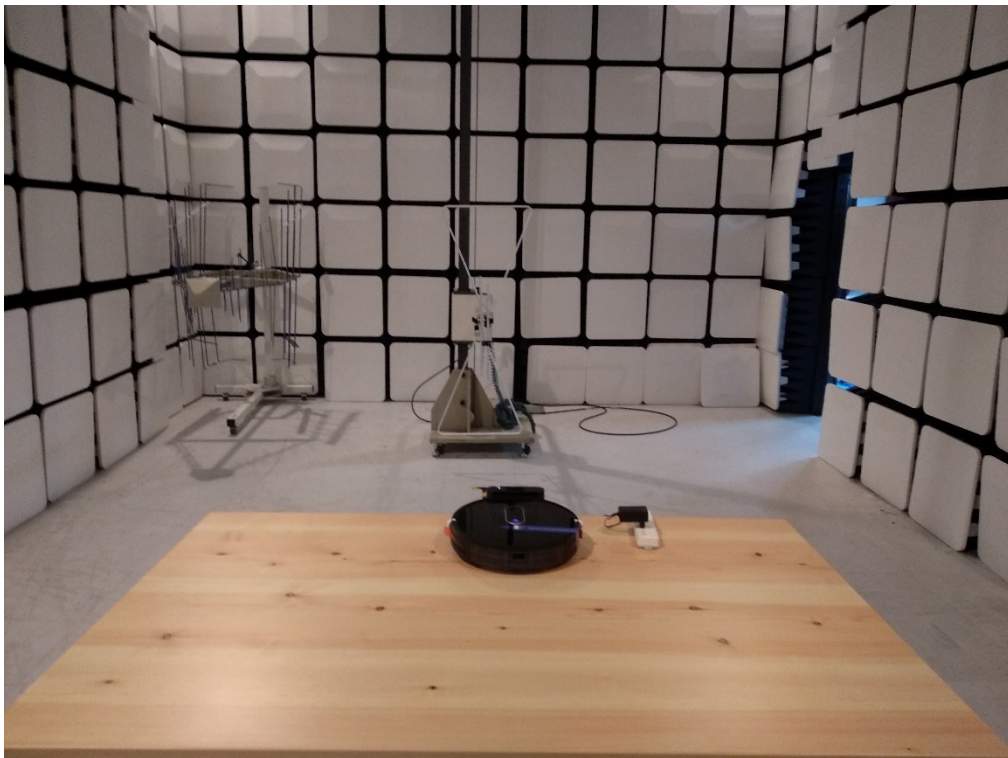
Radiation emission
