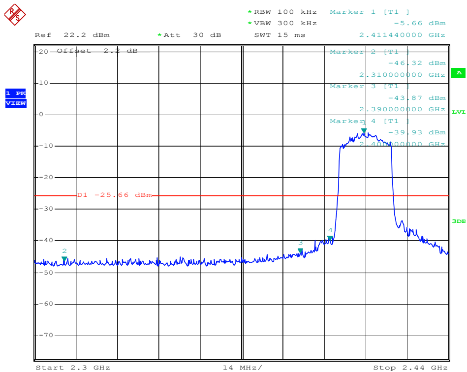
802.11n-HT20-Lowest Lowest
