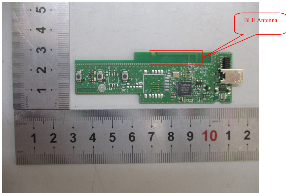
EUT –PCB -1 Chip View
