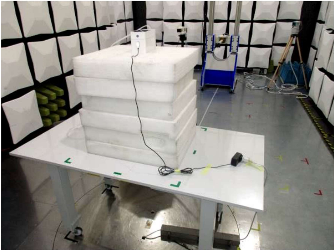
EUT standing
