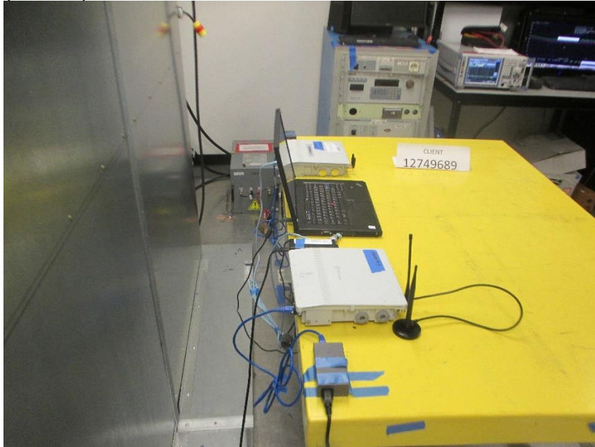
(CLIENT) LINE CONDUCTED BACK PHOTO
