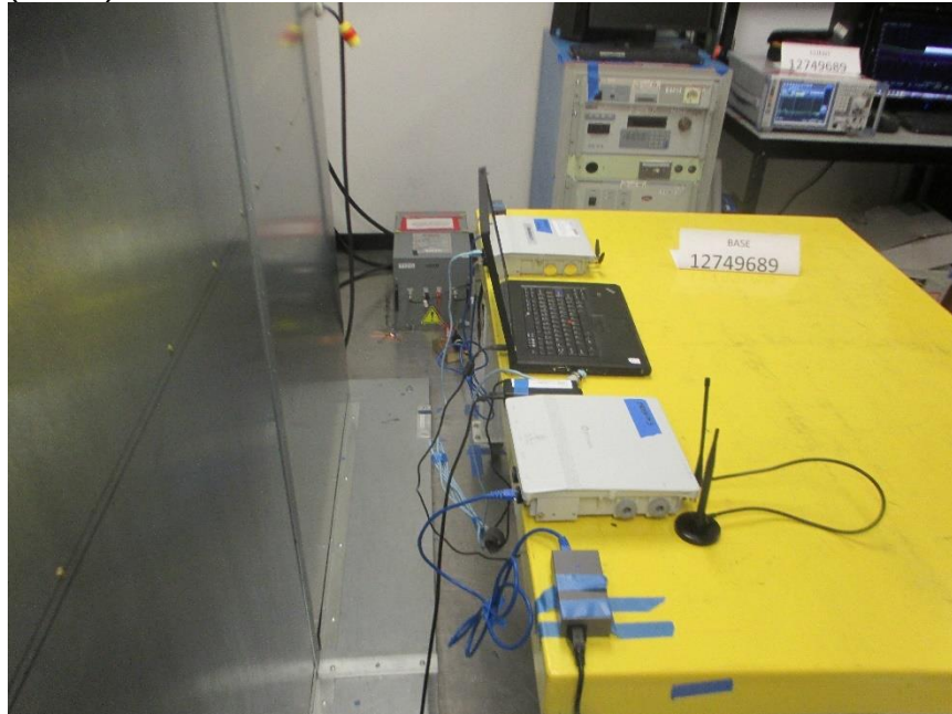
(BASE) LINE CONDUCTED BACK PHOTO
