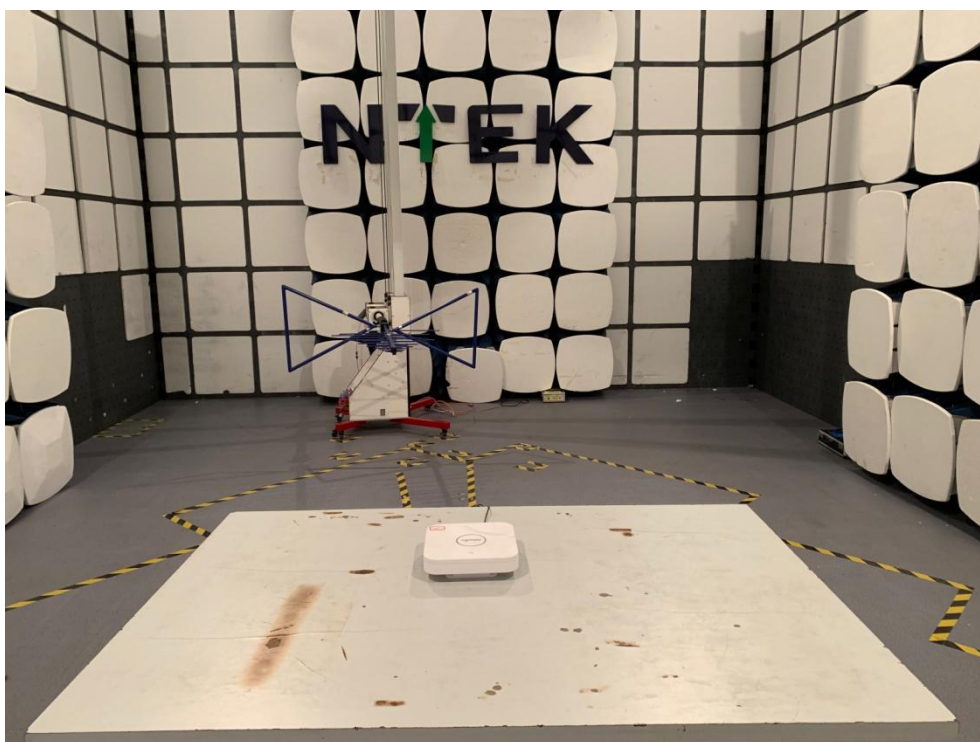
Radiated Measurement Photos(30MHz~1GHz )-Adapter 1
