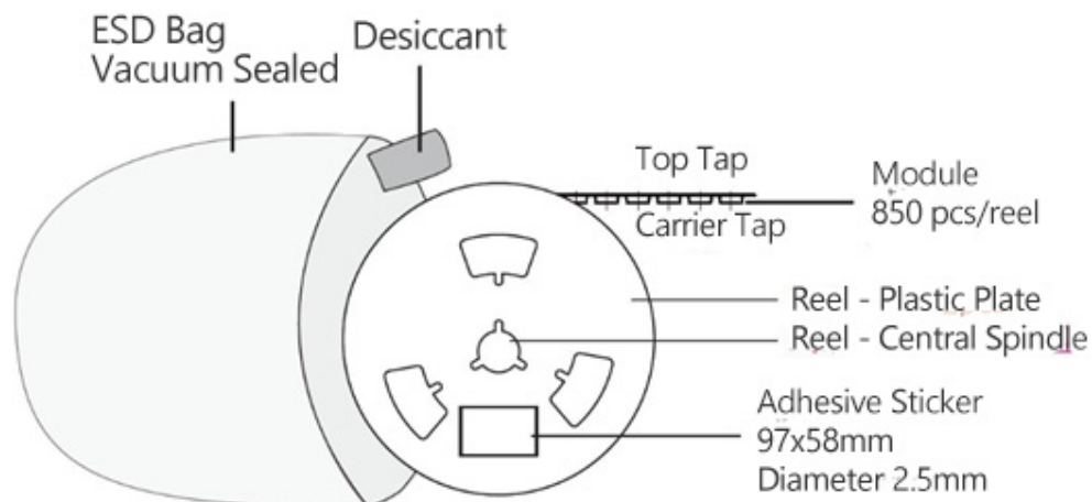
Fig 7 Packaging
