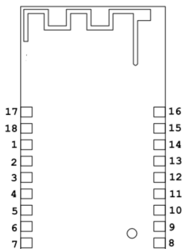
Fig 1 - pin sequence
