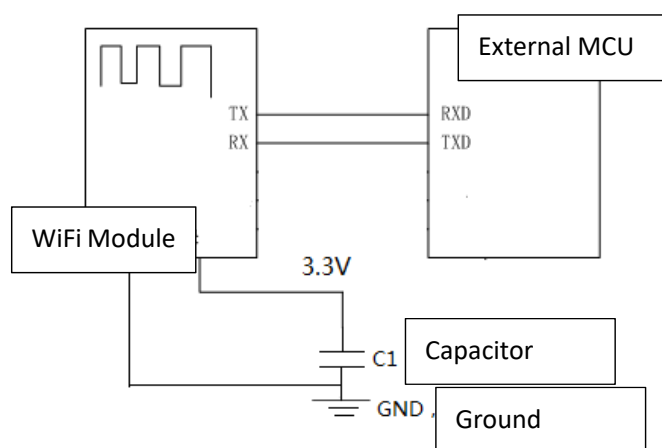
Fig 9 - Circuit Diagram (3.3V)
