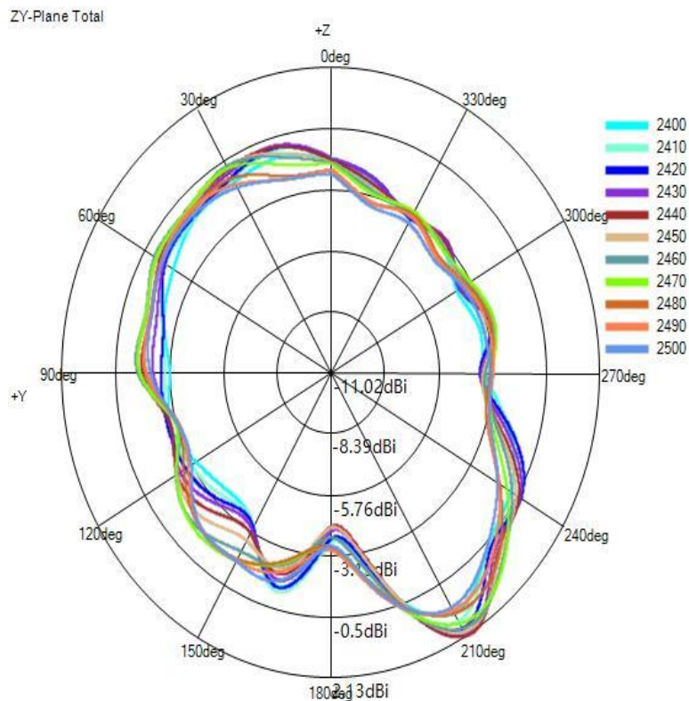
(2) Y-Z Plane(unit:dBi):
