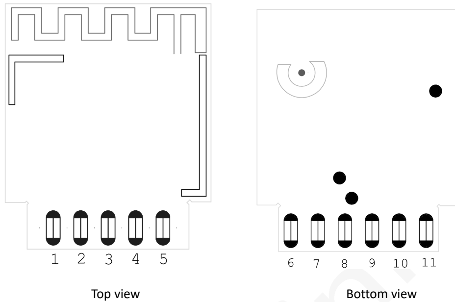
Fig 1 BL33A1-P pin sequence
