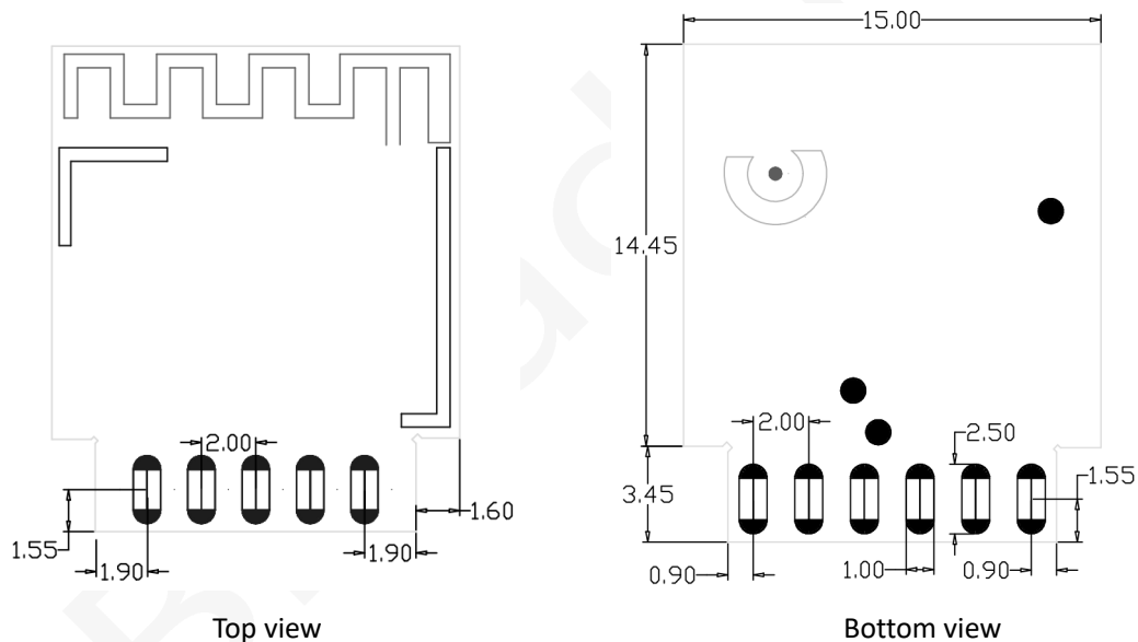
Fig 3 BL33A1-P Module Dimensions
