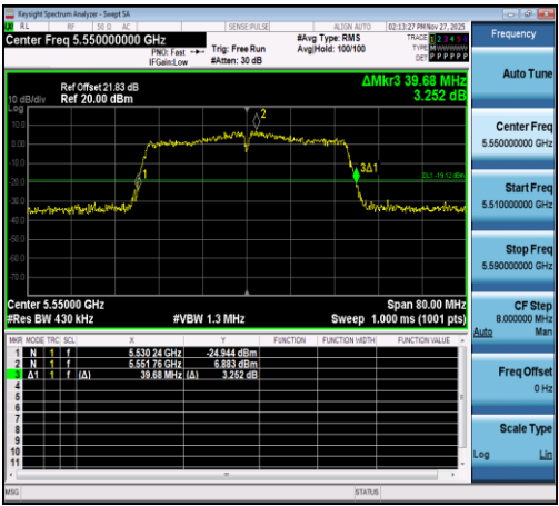
11AC40SISO-Ant1-5550
