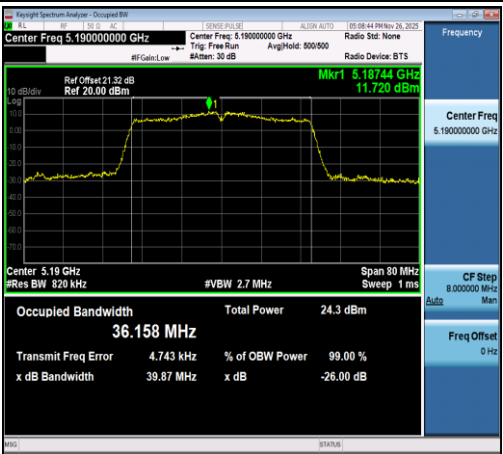
11N40SISO-Ant1-5190
