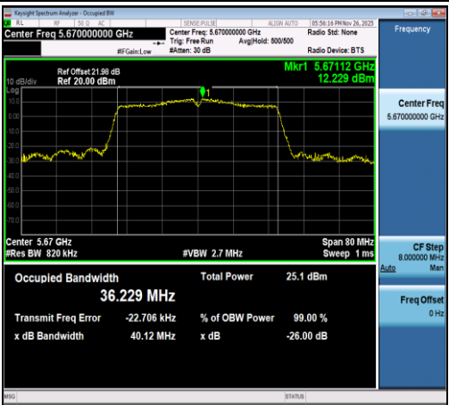
11N40SISO-Ant1-5670
