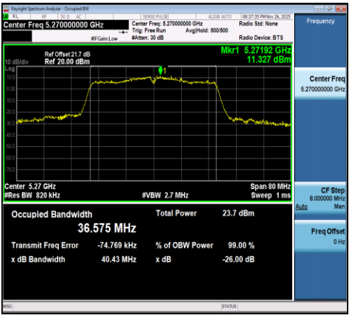
11AC40SISO-Ant1-5270
