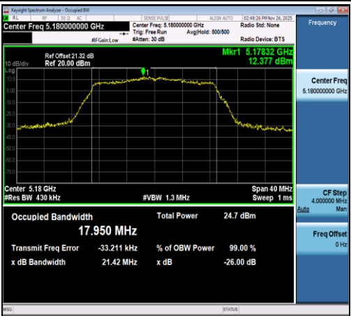
11N20SISO-Ant1-5180
