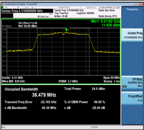
11AC40SISO-Ant1-5310
