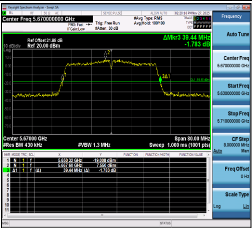
11AC40SISO-Ant1-5670
