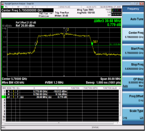
11AC40SISO-Ant1-5795
